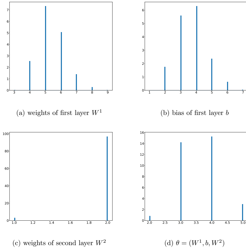
Figure 3.10 – Histogram of the number of eigenvalues given by (3.13) required to reach 0.9 of explained variance (left: weights of the first layer, middle: bias of the first layer, right: weights of the last layer) for spiral data.
