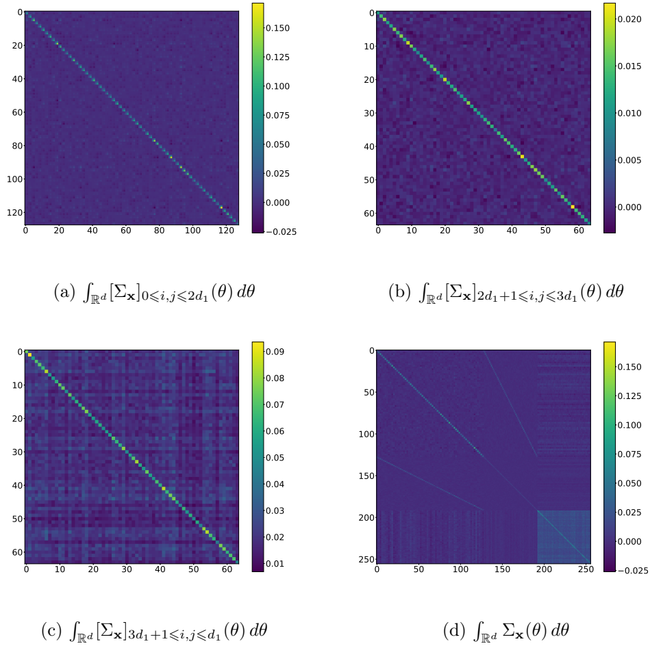
Figure 3.5 – Mean of the covariance matrix of the stochastic estimator \Sigma_{\mathbf{x}} for the toy classification model (top left: weights of the first layer, top right: bias of the first layer, bottom left: weights of the last layer, bottom right: full covariance matrix).
