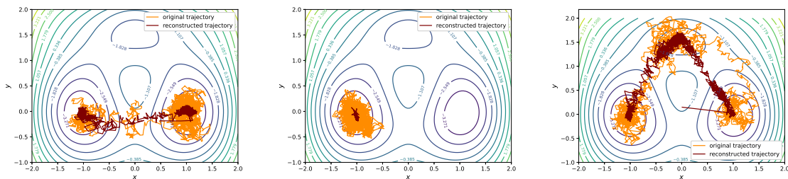
Figure 4.3 – Comparison between original and reconstructed trajectories using the trained "naive" VAE. The orange lines represent the original trajectories (from the test set) and the brown lines the reconstructed ones.
