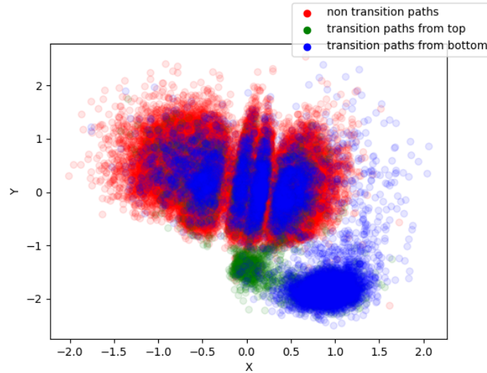
Figure 4.5 – Illustration of the mean embeddings for the test set (using the VAE with embedding space of dimension 31 \times 2 ). Each trajectory is represented by 31 points.
