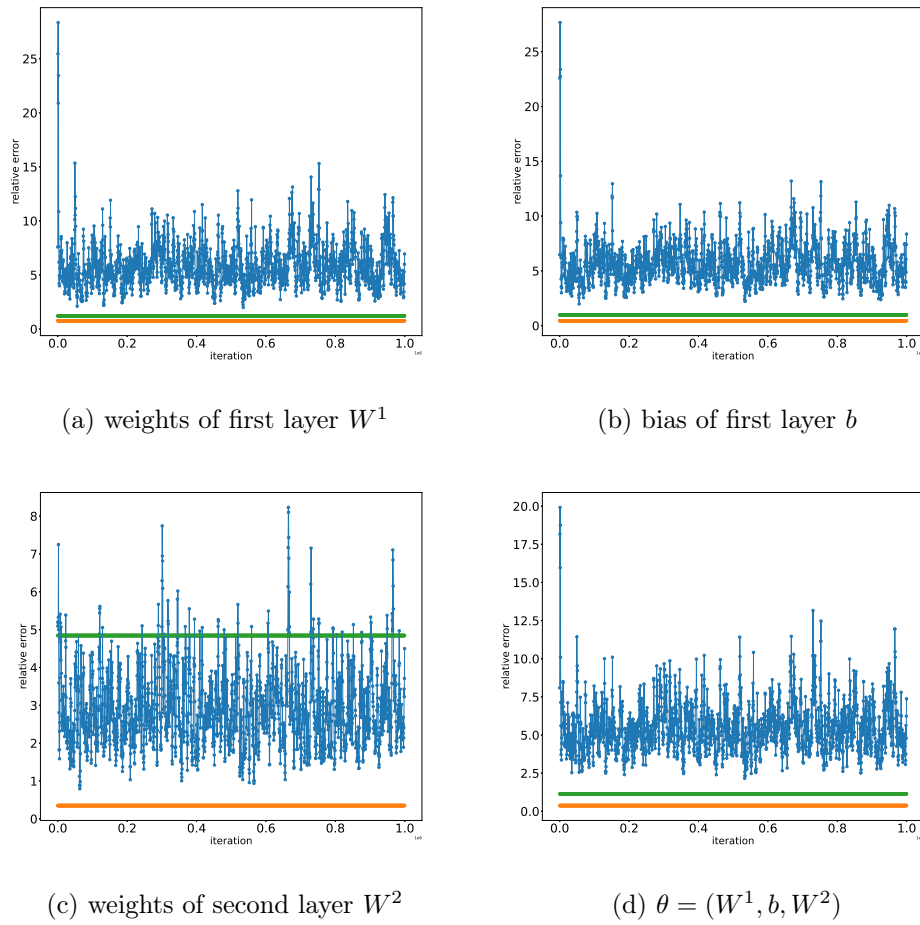
Figure 3.7 – Difference between the covariance matrix and its mean under the posterior measure \pi(\theta|\mathbf{x}) for the toy classification model. The blue line represents the expression (3.10), the orange line represents the expression (3.11) and the green line represents the equation (3.12).
