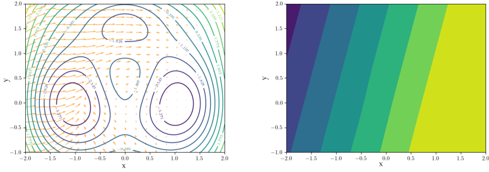
Figure 4.7 – Left: Visualization of the policy \mathcal{P}(q, \omega_f) . The action field "pushes" the simulation from A through the upper saddle point and diminishes in magnitude in the neighborhood of the second metastable region. Right: Visualization of the critic value at a given position for the optimal action, namely \mathcal{Q}(q, \mathcal{P}(q, \omega_f), \theta_f) .
