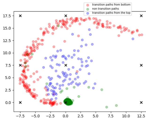
Figure 4.2 – Illustration of the mean embeddings for the test set for the "naive" VAE. The crosses represent the points used to generate new trajectories, see Figure 4.4.
