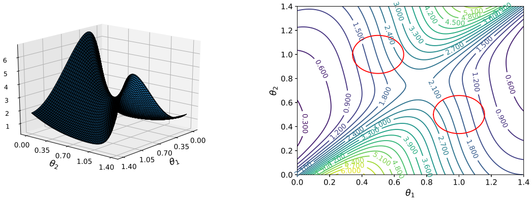
(b) \Sigma_{2,2}
