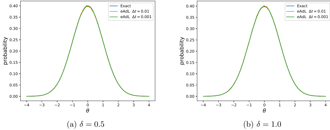
Figure 2.9 – Sampling the Gaussian distribution using the scheme (2.66) for eAdL and various values of \delta . The solid blue line is the exact distribution.
