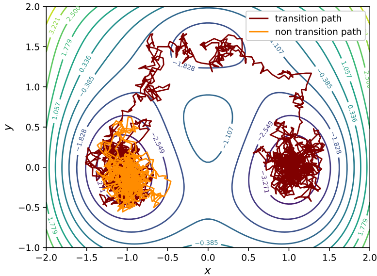
Figure 1.1 – Transition path and non transition path for the 2-dimensional potential given by (4.3).
