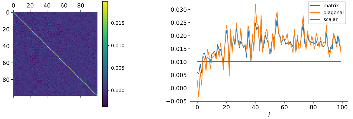
Figure 2.13 – Left: Estimated covariance matrix of \theta . Right: Diagonal components of the estimate of the average covariance matrix of the stochastic gradient as a function of the index 1 \leq i \leq d .
