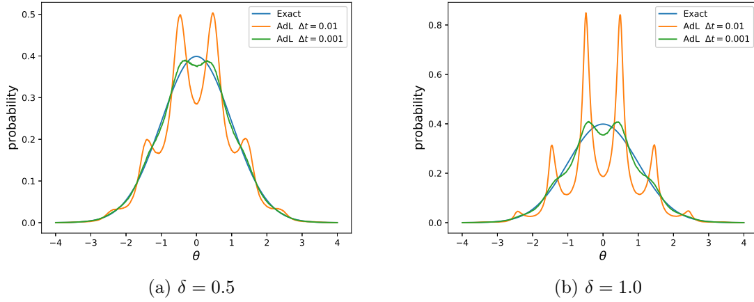
Figure 2.8 – Sampling the Gaussian distribution using the scheme (2.52) for Adaptive Langevin dynamics and various values of \delta . The solid blue line is the exact distribution.
