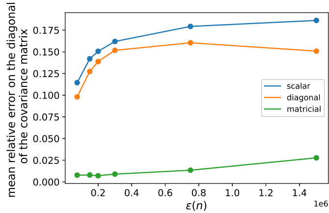
Figure 2.14 – Error on the covariance matrix of the parameters using AdL for \xi scalar, diagonal matrix or full matrix.
