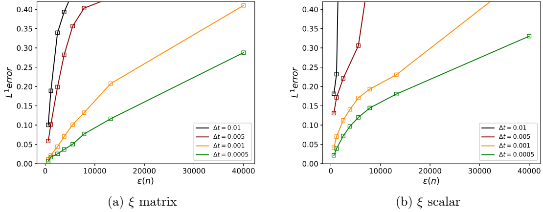
Figure 2.7 – L^1 error on the posterior distribution for various values of \Delta t and n when sampling from the posterior distribution for the mixture of Gaussians case using AdL, with mini-batching performed without replacement.
