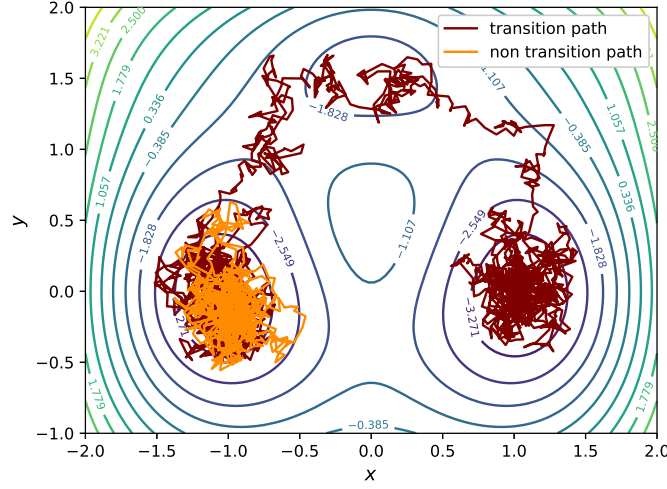
Figure 4.1 – Transition path and non transition path in the 2-dimensional potential given by (4.3).
