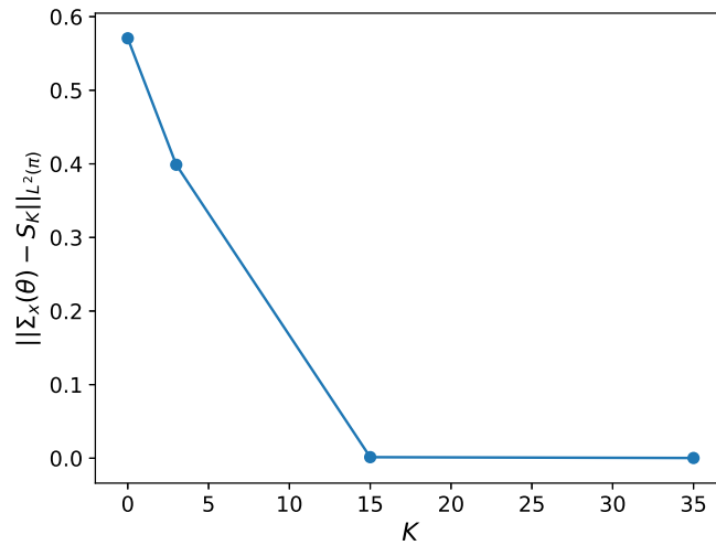
Figure 2.11 – \|\Sigma_{\mathbf{x}} - S_K\|_{L^2(\pi)} where S_K is the L^2(\pi) projection of \Sigma_{\mathbf{x}} onto the vector space of symmetric matrices generated by the basis for each value of K .
