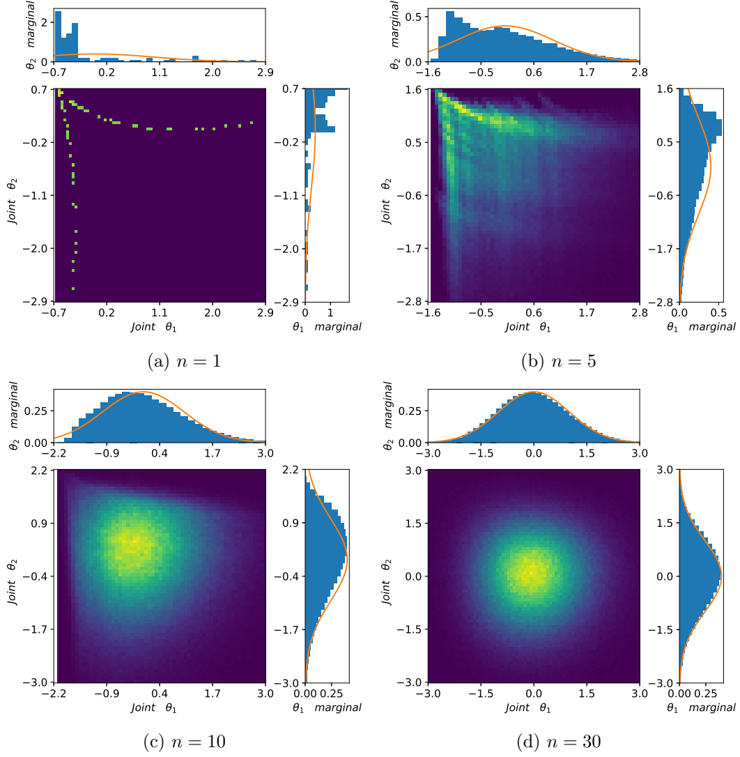
Figure 2.2 – Histogram of Z_{\mathbf{x}, N_{\text{data}}, n} for \theta = (1, 0.2) , when sampling is performed without replacement for the model of Section 2.2.5.2 with N_{\text{data}} = 100 data points sampled from a mixture of Gaussians with parameters \sigma_1 = \sigma_2 = 0.4 , w = 0.5 , \theta_1 = 0.2 and \theta_2 = 1 . The reference standard Gaussian distribution is superimposed as a continuous line on the marginal distributions in \theta_1, \theta_2 .
