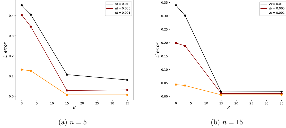
Figure 2.10 – L^1 error on the the marginal over \theta_1 of the a posteriori distribution with eAdL for various values of K and \Delta t ( K = 0 corresponds to AdL results).
