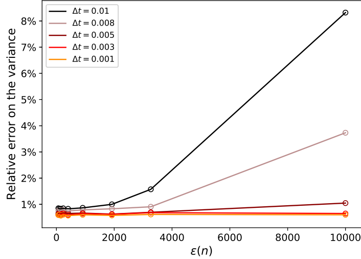
Figure 2.5 – Relative error on the variance of the posterior distribution for various values of n using AdL when the elementary likelihood is Gaussian, and sampling is performed without replacement.
