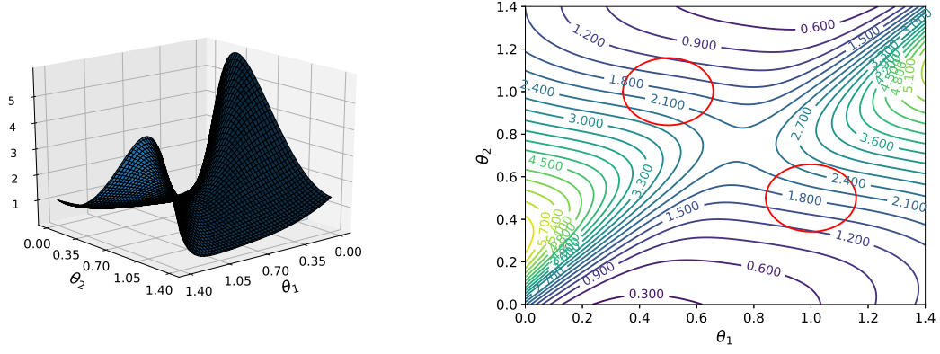
(a) \Sigma_{1,1}
