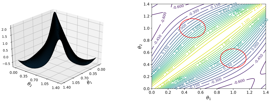
(c) \Sigma_{1,2}
