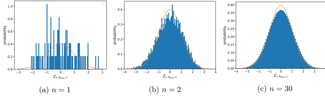
Figure 2.1 – Histogram of Z_{\mathbf{x}, N_{\text{data}}, n} when sampling is performed without replacement for the Gaussian model of Section 2.2.5.1, with N_{\text{data}} = 100 , \sigma_\theta = 1 , \sigma_x = 1 , \mu = 0 , \theta = 0.5 . The reference standard Gaussian distribution is superimposed as a continuous line.
