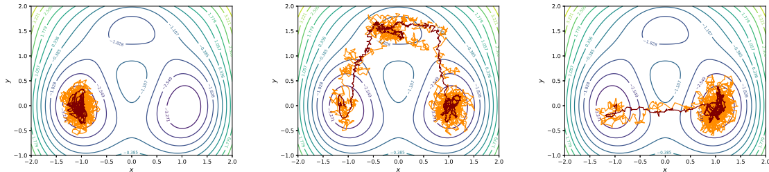
Figure 4.6 – Comparison between original and reconstructed trajectories using the trained VAE with an embedding space of dimension 31. The orange lines represent the original trajectories (from the test set) and the brown lines the reconstructed ones.
