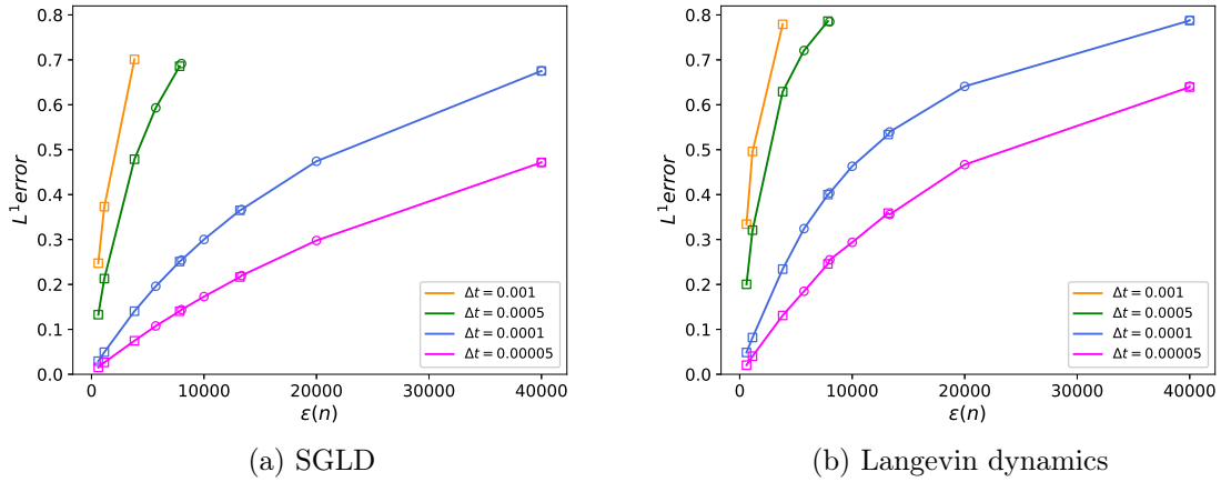
Figure 2.4 – L^1 error on the \theta_1 marginal of the posterior distribution for various values of \Delta t and n when the elementary likelihoods are mixtures of Gaussians, when sampling with (circles) and without replacement (squares).
