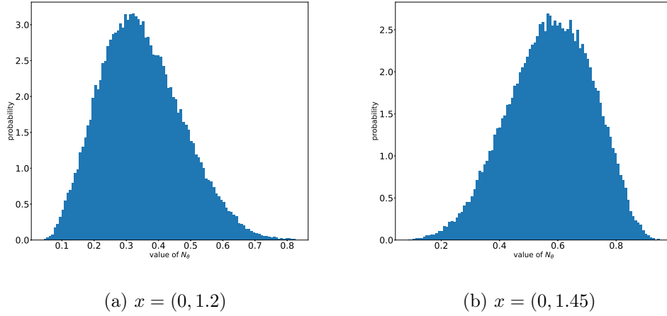
Figure 3.14 – Histogram of N_\theta(x) for various values of x .
