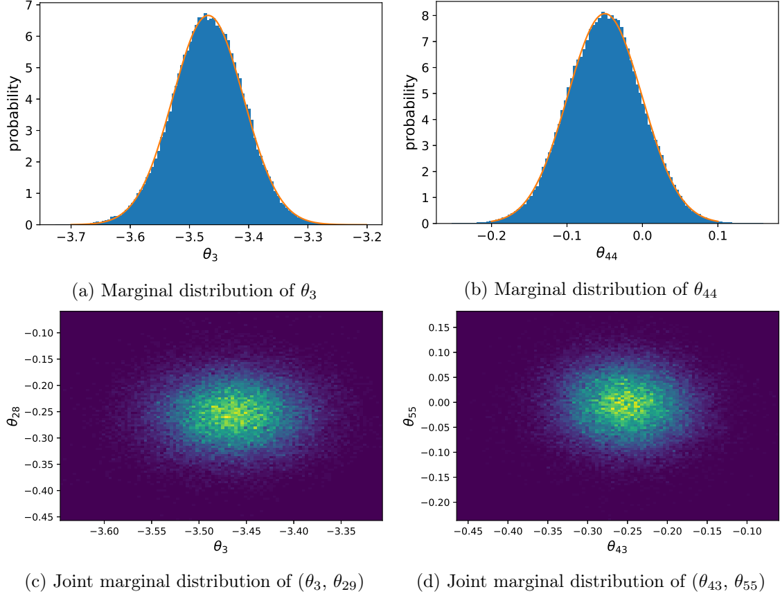
Figure 2.12 – Marginal posterior distributions of \theta_3 and \theta_{44} (top), and of (\theta_3, \theta_{28}) and (\theta_{43}, \theta_{55}) (bottom).
