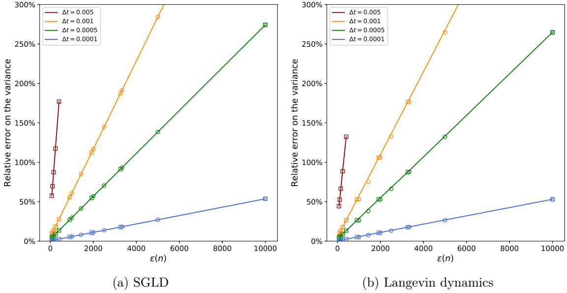
Figure 2.3 – Relative error on the variance of the posterior distribution for various values of \Delta t and n when the elementary likelihood is a Gaussian distribution, when sampling with (circles) and without replacement (squares).
