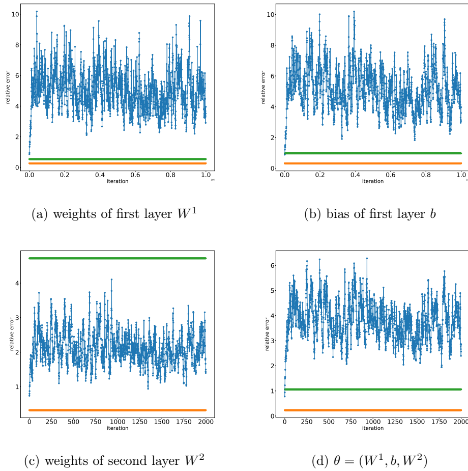
Figure 3.6 – Difference between the covariance matrix and its mean under the posterior measure \pi(\theta|\mathbf{x}) for the spiral data case. The blue line represents the expression (3.10), the orange line represents the expression (3.11) and the green line represents the equation (3.12).
