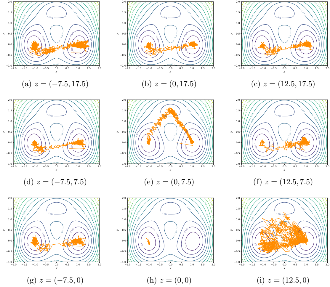
Figure 4.4 – Generated trajectories using the trained "naive" VAE, for various values of the latent variables (see crosses in Figure 4.2).
