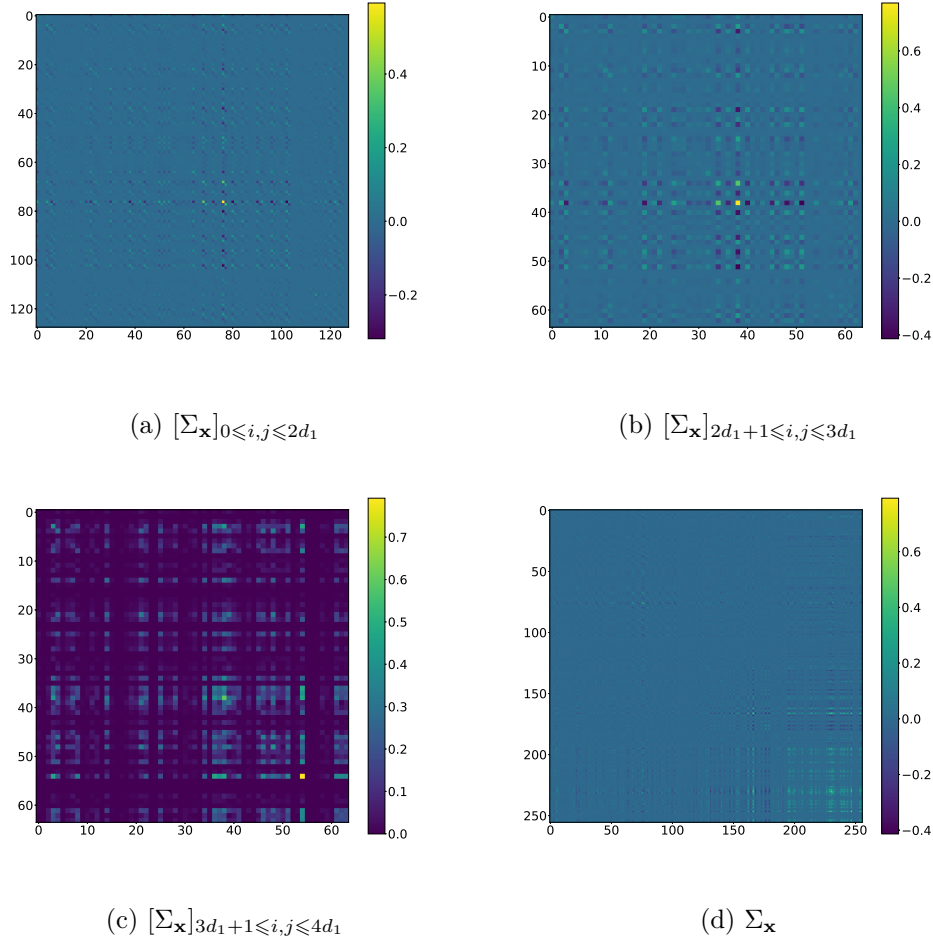
Figure 3.3 – Covariance matrix of the stochastic estimator \Sigma_{\mathbf{x}} at iteration 5 \times 10^5 for the spiral data case (top left: weights of first layer, top right: bias of first layer, bottom left: weights of the second layer, bottom right: full covariance matrix).
