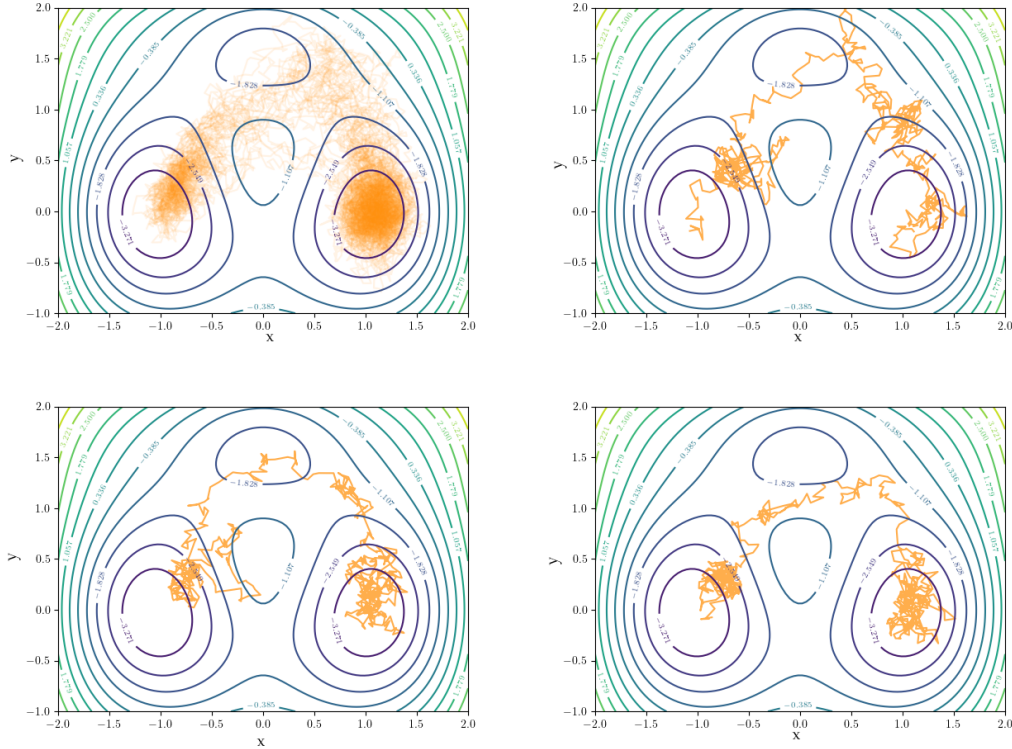
Figure 4.8 – Sample trajectories generated using (4.26) (one per picture, except the top left in which 25 trajectories are represented).
