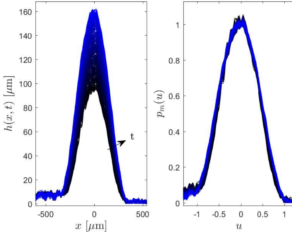
Figure 39: Time evolution of the interface profile h(x, t) of the droplet deformation in a "mechanical" device in which d_z = 5 \mu\text{m} , d_x = 400 \mu\text{m} , e = 30 \mu\text{m} and w = 400 \mu\text{m} . The droplet is 1600 \mu\text{m} long. The timelapse that is plotted is around 70s. During this period of time, h(x, t) is self-similar and writes h(x, t) = h_0(t)p(x) . We define u = x/b where b is the x -axis extent of the neck that is constant over time.
