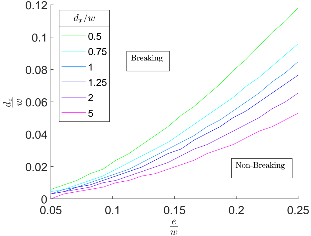
Figure 43: Phase diagram that predicts the fate of droplets in devices with dimensions (e, w, d_z, d_x) : breaking (above the line) or non-breaking (below the line). The geometric parameters are adimensionned by the channel width w . The curves correspond to the spectrum of equations w - 2h_{eq} = e plotted for different ratios \frac{d_x}{w} .
