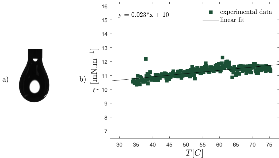
Figure 26: a) Image of a pendant drop b) Profile of the interfacial tension between mineral oil and water mixed for [SDS]=2 CMC.
