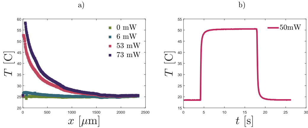
Figure 18: a) Spatial temperature profile measured with an infrared camera for 0 < P < 75 mW along the x -axis. b) Temporal temperature profile for P = 50 mW. The resistance is switched on at t = 4.6 s and off at t = 18.5 s .
