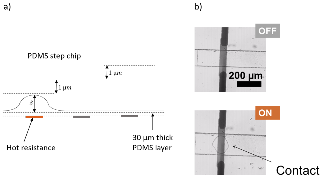
Figure 21: a) Scheme of the home-made calibration step device. The device contains steps in its roof to measure the dilation of micro-channels. The channel width is 200µm and its height is comprised in between 1 and 15 µm with steps of 1 µm. b) Typical observation that is made in the calibration chip. A contact line appears when the channel walls dilate such that the top wall touches the bottom wall.
