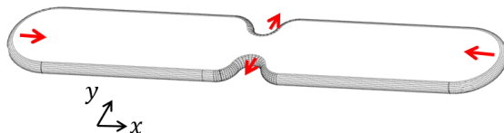
Figure 66: Direction of the moving droplet menisci in the neck region and at the extremities of the droplet.
