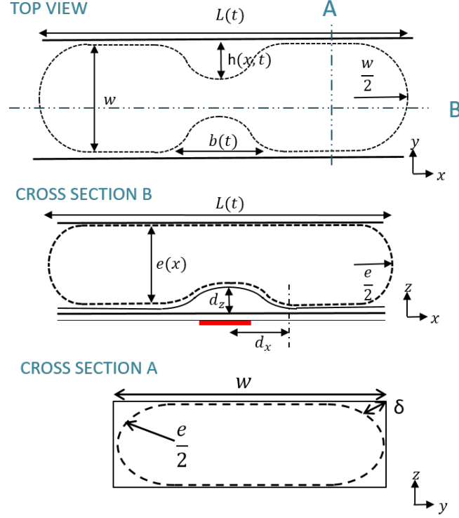
Figure 36: Geometrical parameters that are used to describe the droplet deformation.
