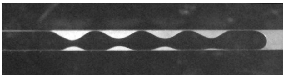
Figure 53: Droplet deformed by a succession of confinement gradient indented in a system made out of a micro-milled mold.
