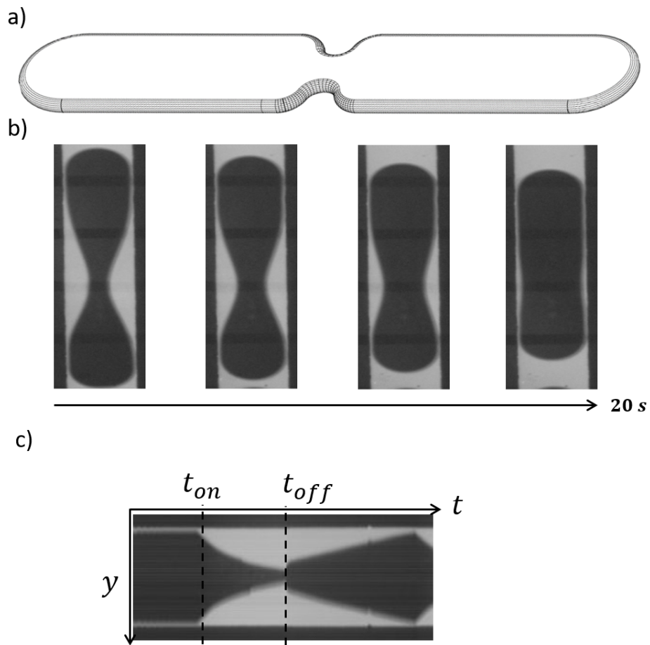
Figure 55: a) 3D illustration of the peanut-like shape droplet b) Snapshot of a 800\ \mu\text{m} long droplet relaxation in a 200\ \mu\text{m} \times 30\ \mu\text{m} rectangular channel. The images are displayed every 5 seconds. c) Spatio-temporal evolution of the neck width during the droplet deformation t_{on} < t < t_{off} and the droplet relaxation t > t_{off} . t_{on} is the time at which the resistance is switched on and t_{off} is the time at which the resistance is switched off.
