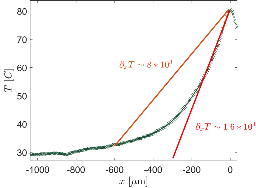
Figure 19: Spatial evolution of the temperature profile. Upper (red) and lower bound (orange) of the temperature gradient for T = 80 °C.
