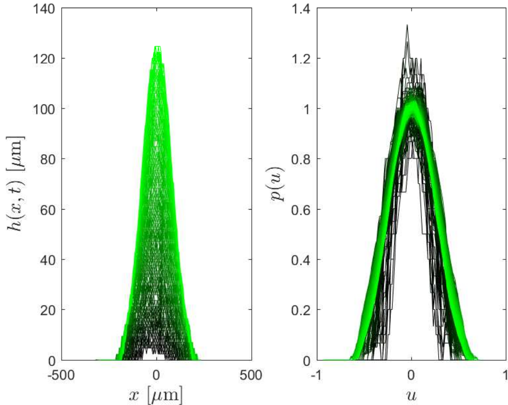
Figure 72: (a) Interface profile h(x, t) at the level of the neck during the entire process of the droplet deformation. b) Associated self-similar function p_r as a function of u = x/b .
