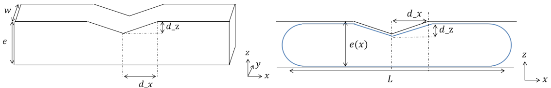
Figure 37: Scheme of a mechanical device in which a confinement gradient is indented. The system is called the "mechanical" system and is compared to the "thermomechanical" system. a) 3D view b) Cross view in the plane (x, z) .
