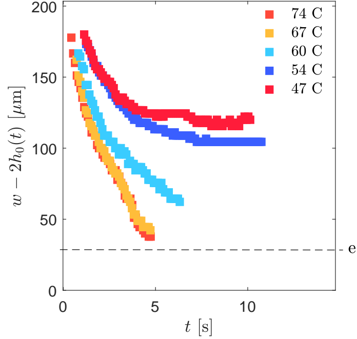
Figure 31: Time evolution of the neck width for a large range of temperature ( 47\text{ }^{\circ}\text{C} < T < 74\text{ }^{\circ}\text{C} ). Given the conditions of the experiment ( 800\text{ }\mu\text{m} long droplet in a 30\text{ }\mu\text{m} and 200\text{ }\mu\text{m} high and wide channel), we can assume that the critical temperature T^* above which the droplet breaks is comprised in between 54\text{ }^{\circ}\text{C} and 60\text{ }^{\circ}\text{C} .
