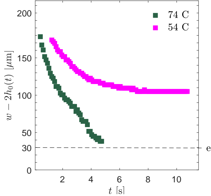
Figure 30: Time evolution of the neck width for a non-breaking and for a breaking droplet. In this experiment, the droplet length is 800 \mu\text{m} , the channel height and width are respectively 30 \mu\text{m} and 200 \mu\text{m} . For T = 74 °C, the neck width w - 2h_0(t) decreases over time until it reaches the value e = 30 \mu\text{m} and the droplet breaks. For T = 54 °C, the neck width decreases until it reaches a plateau value that is approximately half of the channel width.
