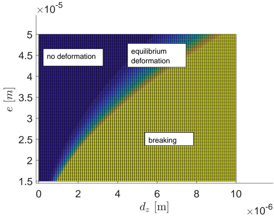
Figure 42: Phase diagram of (e, d_z) for d_x = 400 \mu\text{m} and w = 400 \mu\text{m} , that predicts the fate of droplets in devices with dimensions (e, w = 400, d_z, d_x = 400) : breaking (below the orange line) or non-breaking (above the orange line). A transient region is plotted above the orange line and corresponds to situations in which droplets deform but reach an equilibrium shape. Then, a darker zone is plotted that corresponds to cases in which droplets do not deform.
