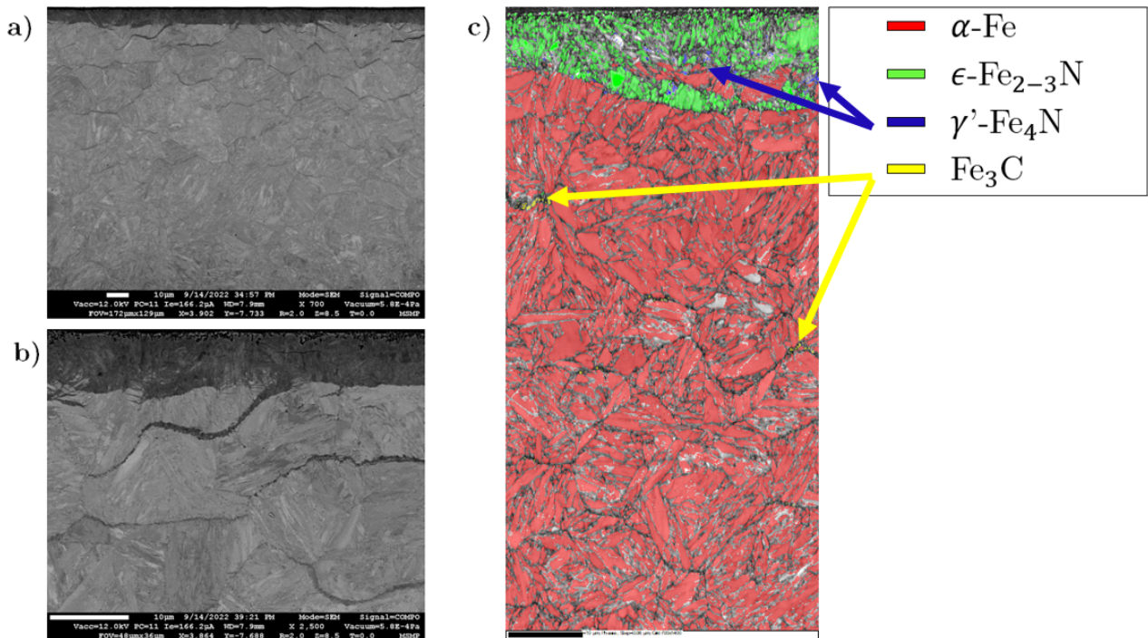
Figure 4.26 – a) BSE image \times 800 , b) BSE image \times 2500 c) EBSD cartography, of 33CrMoV12-9 specimens 1+1 sides (F2) nitrided, of 500 μm thick, at 520 °C with K_N = 3.711 \text{ atm}^{-1/2} during 5 h.
