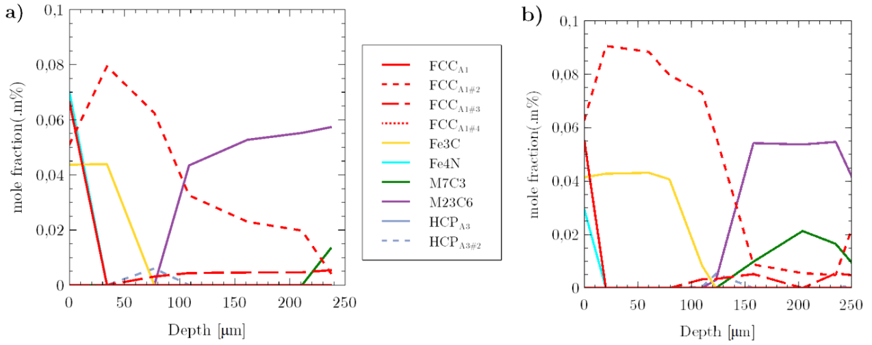
Figure 4.25 – Evolution of the mole fractions of nitrides and carbides obtained in steel grade 33CrMoV12-9 for a) a 5 mm thick (S) nitrided sample and b) a 500 μm thick (F2) nitrided sample.
