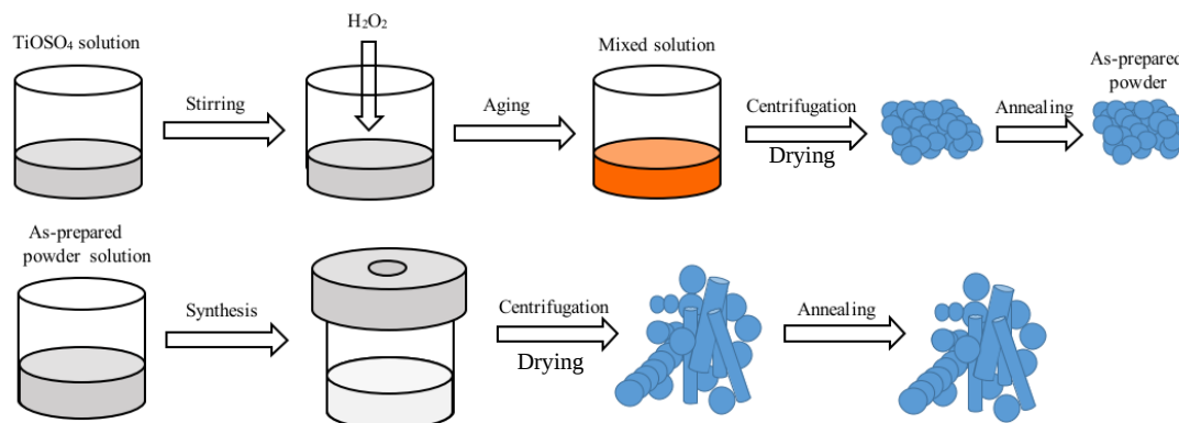
Scheme 1. Schematic illustration of different steps of TiO 2 powder synthesis.
