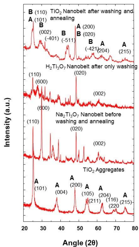
Figure 11 . XRD pattern of \text{TiO}_2 nanobelt at different synthesis stages as indicated and at the synthesis temperature of 100 °C (A: Anatase; B: \text{TiO}_2 -B).
