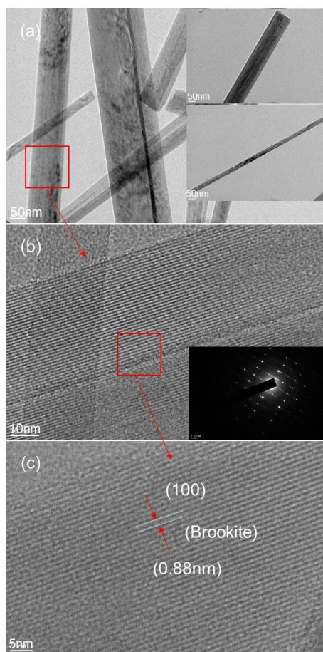
Figure 5 . (a) TEM images of \text{TiO}_2 nanobelt obtained at synthesis temperature of 200^\circ\text{C} a synthesis time of 6 h at different magnifications; (b) the corresponding HRTEM showing inter atomic crystallographic planes and the insert show the corresponding electron diffraction; (c) another magnification of \text{TiO}_2 nanobelt.
