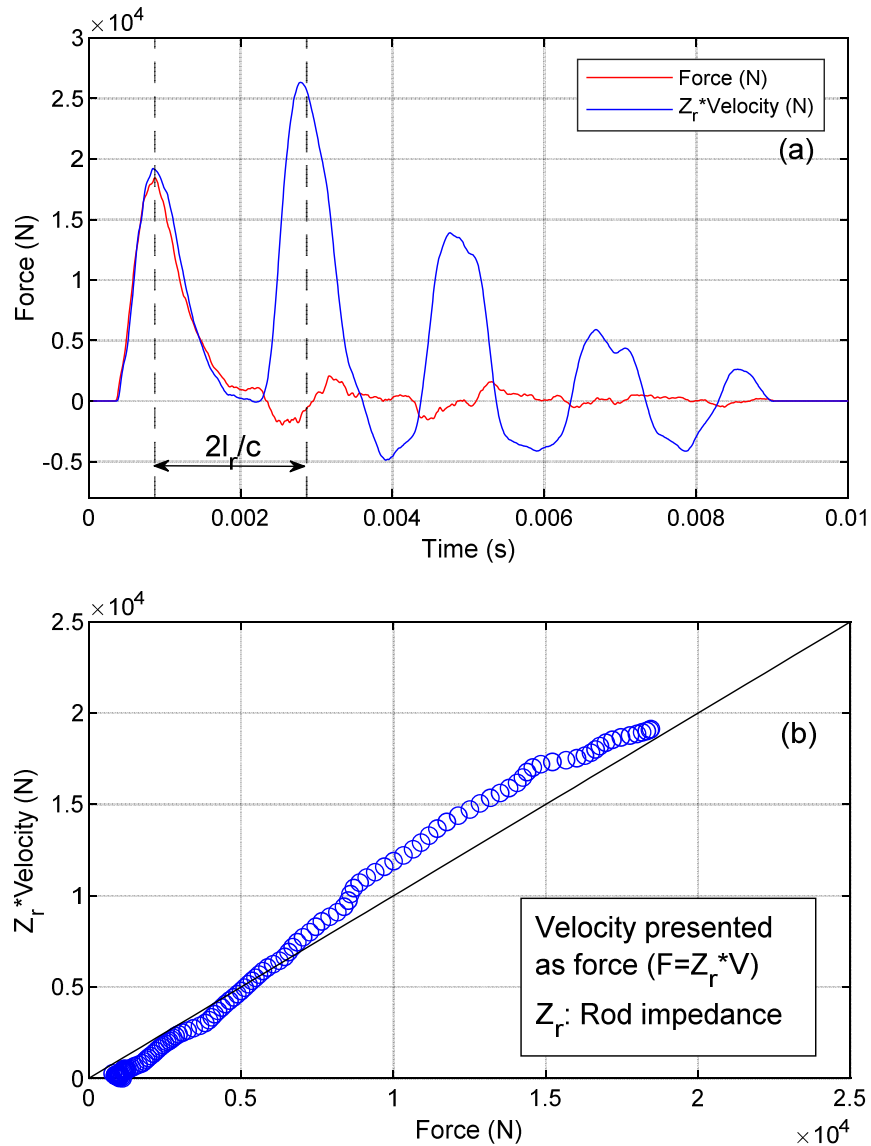
Figure 2-6 – Dynamic force and velocity ( Z \cdot V ) measurements for a set of 4 m rods.
