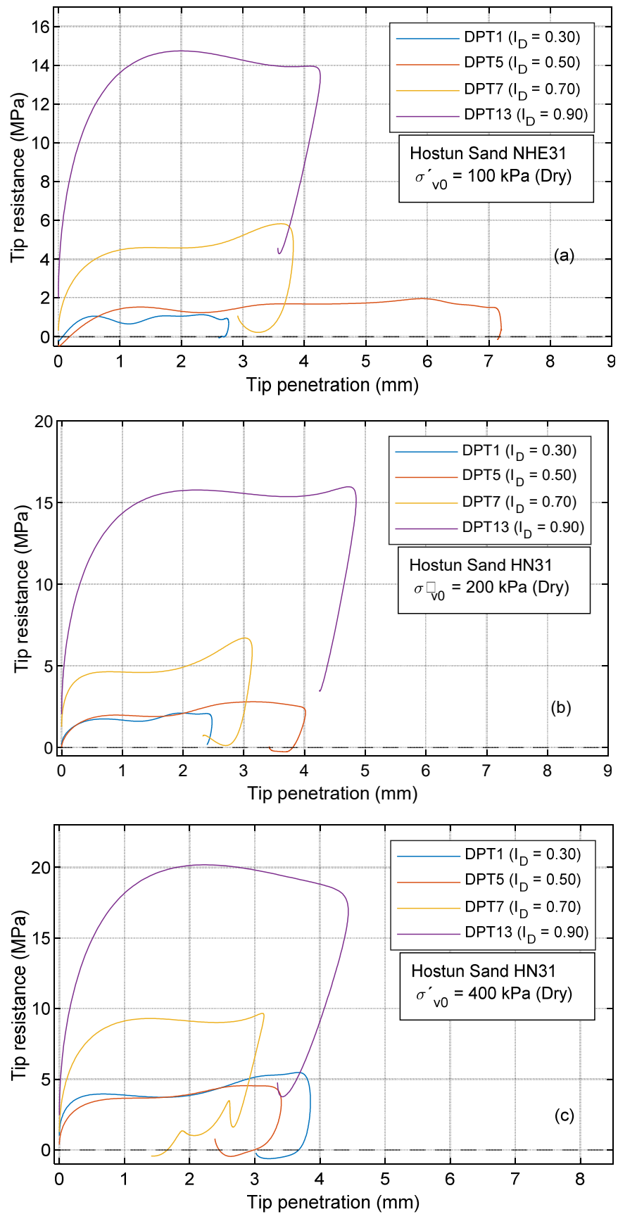
Figure 3-22 – DCLT curves obtained for dry Hostun HN31 sands: combined influence of density index I_D and vertical consolidation stress \sigma'_{v0} .
