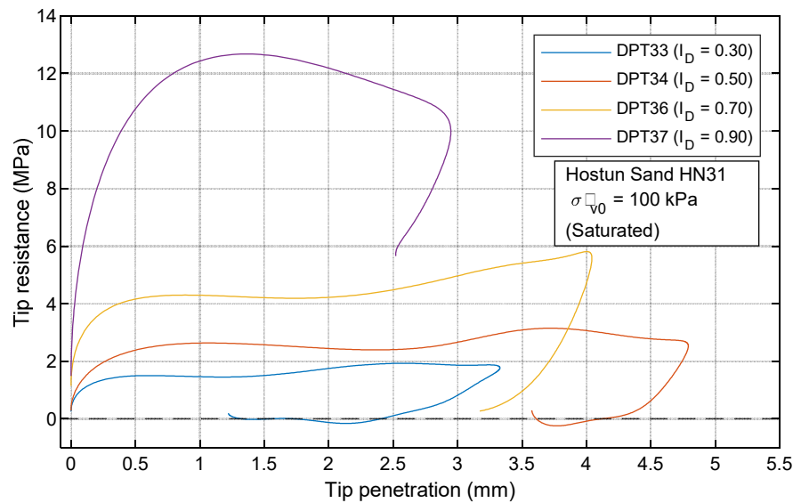
Figure 3-24 – DCLT curves for specimens in saturated Hostun HN31 sands \sigma'_v = 100 \text{ kPa} .
