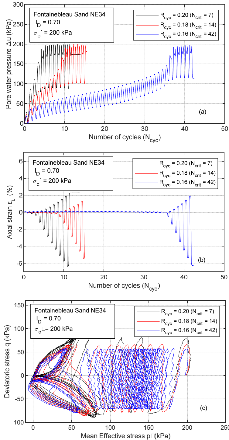
Figure 4-13 – Cyclic stress ratio influence on dense Fontainebleau NE34 sands: (a) excess pore water pressure generation; (b) \epsilon_u - N_{cyc} curve; (c) effective stress path in the (q - p') plane.
