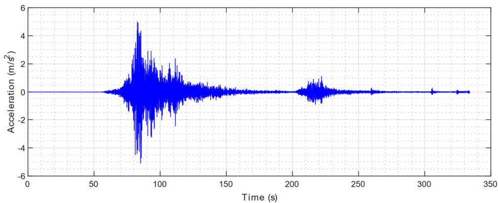
Figure 1-20 - Seismic acceleration measurements (Iquique earthquake 2014) (CSN 2014).
