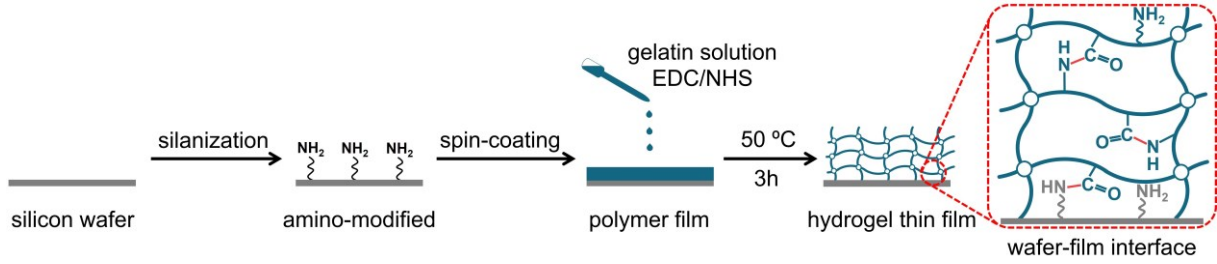
Figure 1. Synthesis process of surface-attached gelatin hydrogel thin films using the CLAG strategy. The CLAG strategy consists in Cross-Linking and Grafting gelatin chains onto the amino-modified silicon wafers with EDC/NHS coupling.
