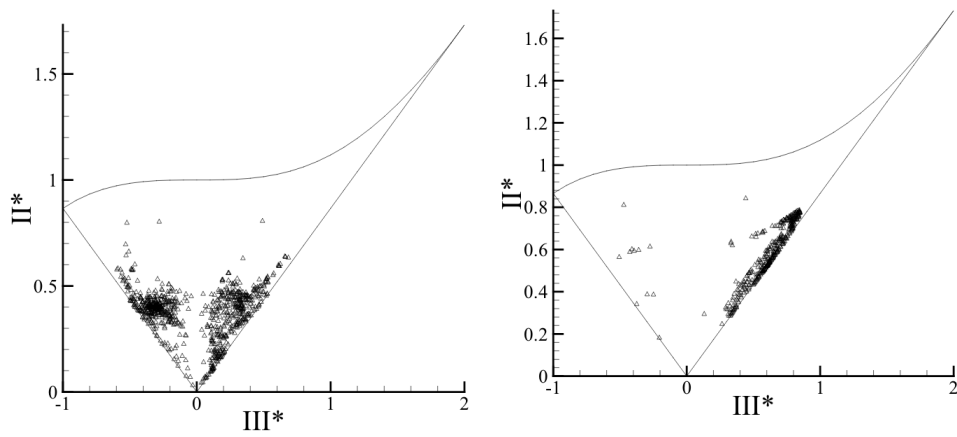
Figure 3.70: Lumley triangles from Kuznik (2005) for the cold jet case. (Left) k - \varepsilon simulation. (Right) R_{ij} - \varepsilon simulation.
