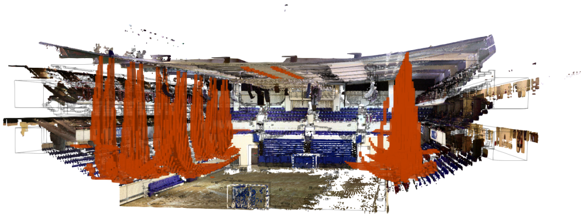
Figure 5.4.4: Volumes with a velocity magnitude higher than 0.5 \text{ m s}^{-1} (red) for the isothermal ventilation case at t = 3000 s.
