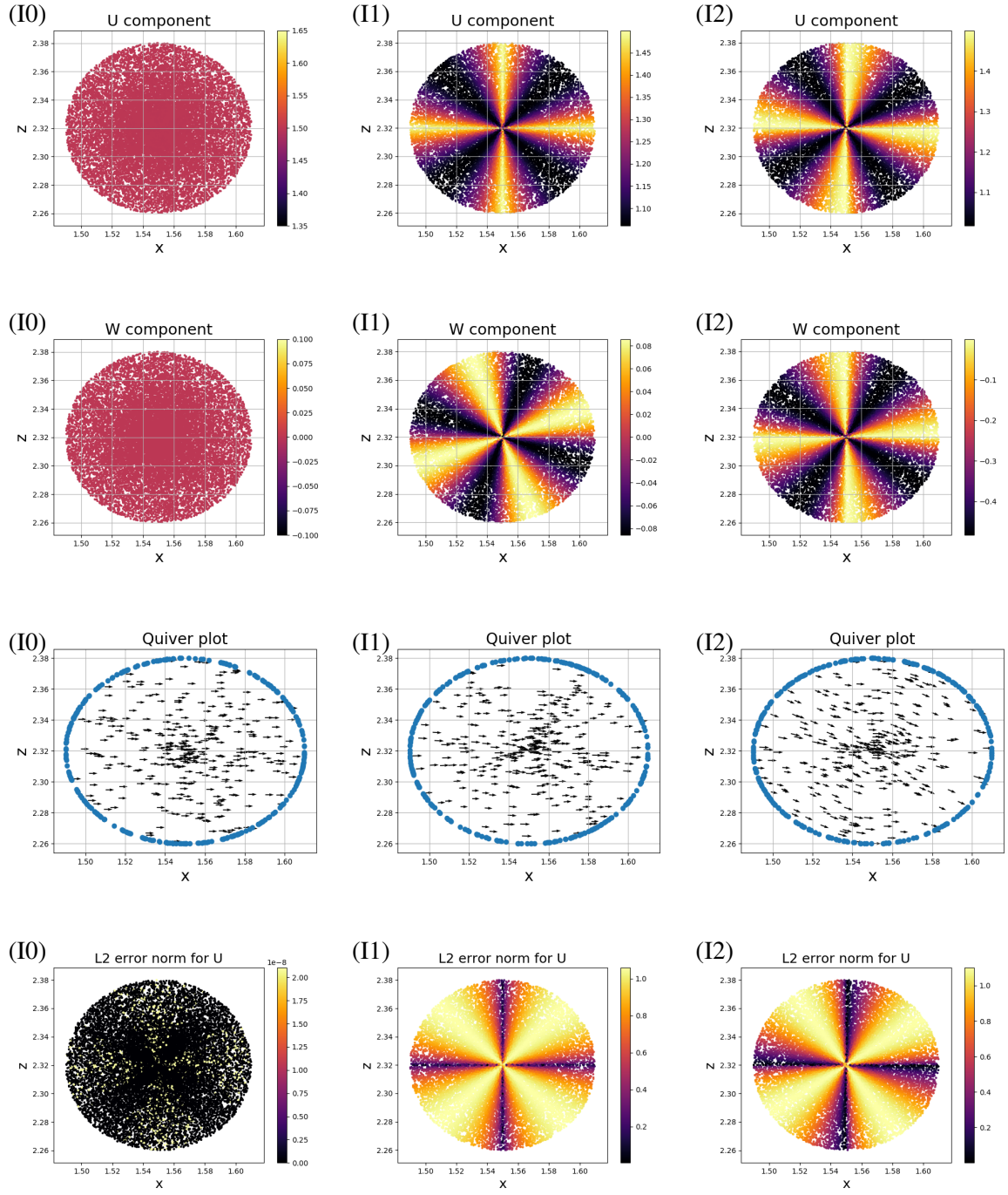
Figure 3.F.3: Second test case. Velocity components fields, quiver plot and L_2 error norm related to the horizontal velocity for the three different interpolations.
