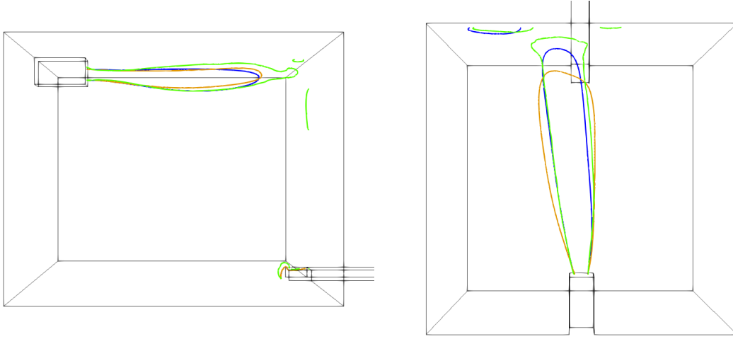
Figure 3.56: Hot jet. Velocity magnitude u_{mag} = 0.4 \text{ m s}^{-1} isoline for all three hot jet simulations. In blue, the k - \varepsilon simulation, in orange, the R_{ij} and in green the LES.
