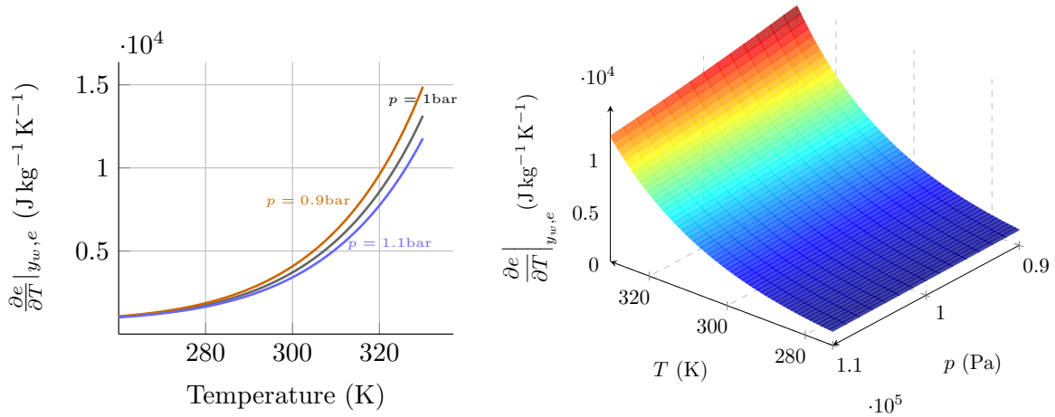
Figure 4.4.1: (Left) 2-D representation of the internal energy partial derivative related to the temperature between 260 K and 330 K for three different pressures in the indoor airflow range and with y_w = 0.0125 . (Right) 3-D representation of the internal energy partial derivative related to the temperature with y_w = 0.0125 .
