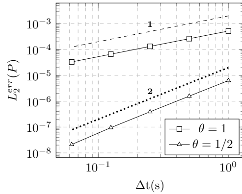
Figure 3.7: Dirichlet boundary condition case. L_2 error norm for the pressure at t = 0.8\tau_2 \text{ s} for a first-order implicit Euler ( \theta = 1 ) and Crank Nicolson ( \theta = 1/2 ) time scheme.
