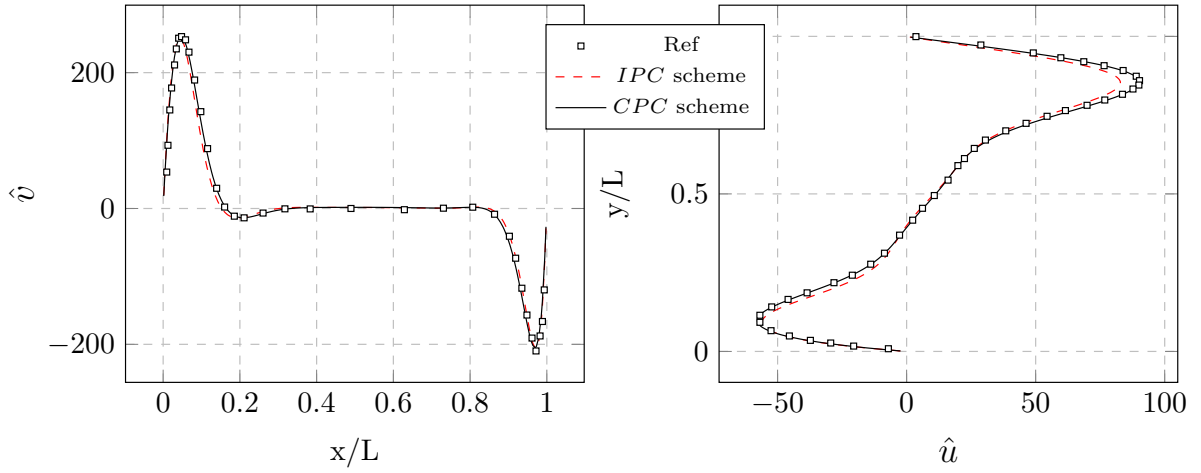
Figure 3.25: Distribution of the velocity on the centrelines of the convective cavity compared to the reference ( Darbandi and Hosseinizadeh, 2006 ).
