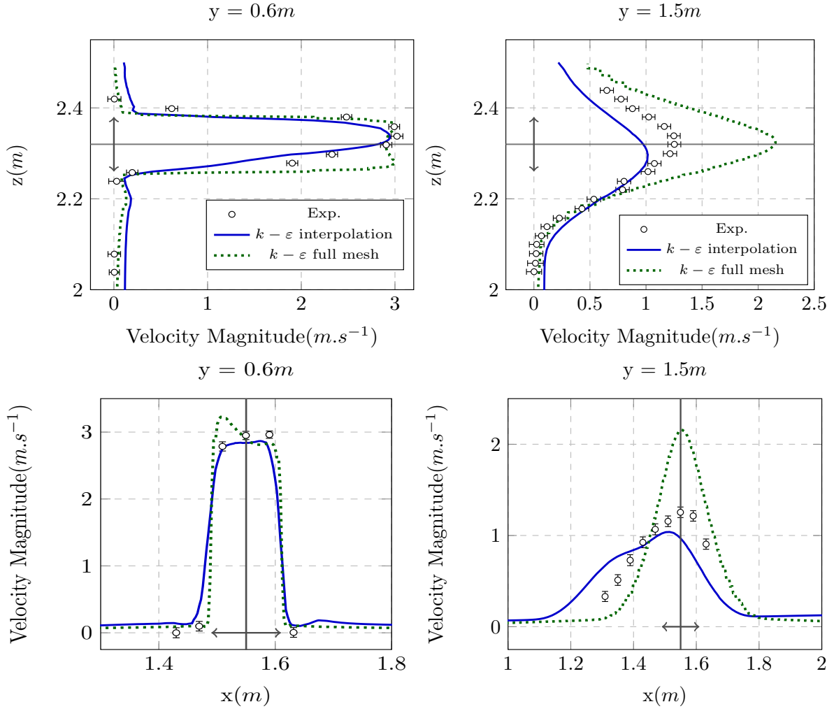
Figure 3.G.3: Vertical (top) and horizontal (bottom) velocity magnitude profiles at y = 0.6\text{ m} and y = 1.5\text{ m} for the full mesh simulation and the inlet interpolation simulation.
