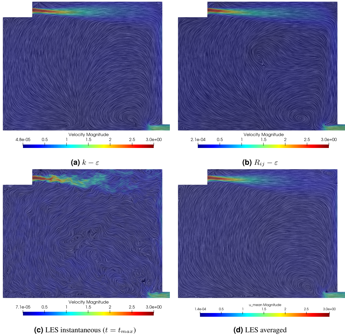
Figure 3.47: Isothermal jet. Velocity magnitude field over the axis x = 1.55 m for the three simulations.
