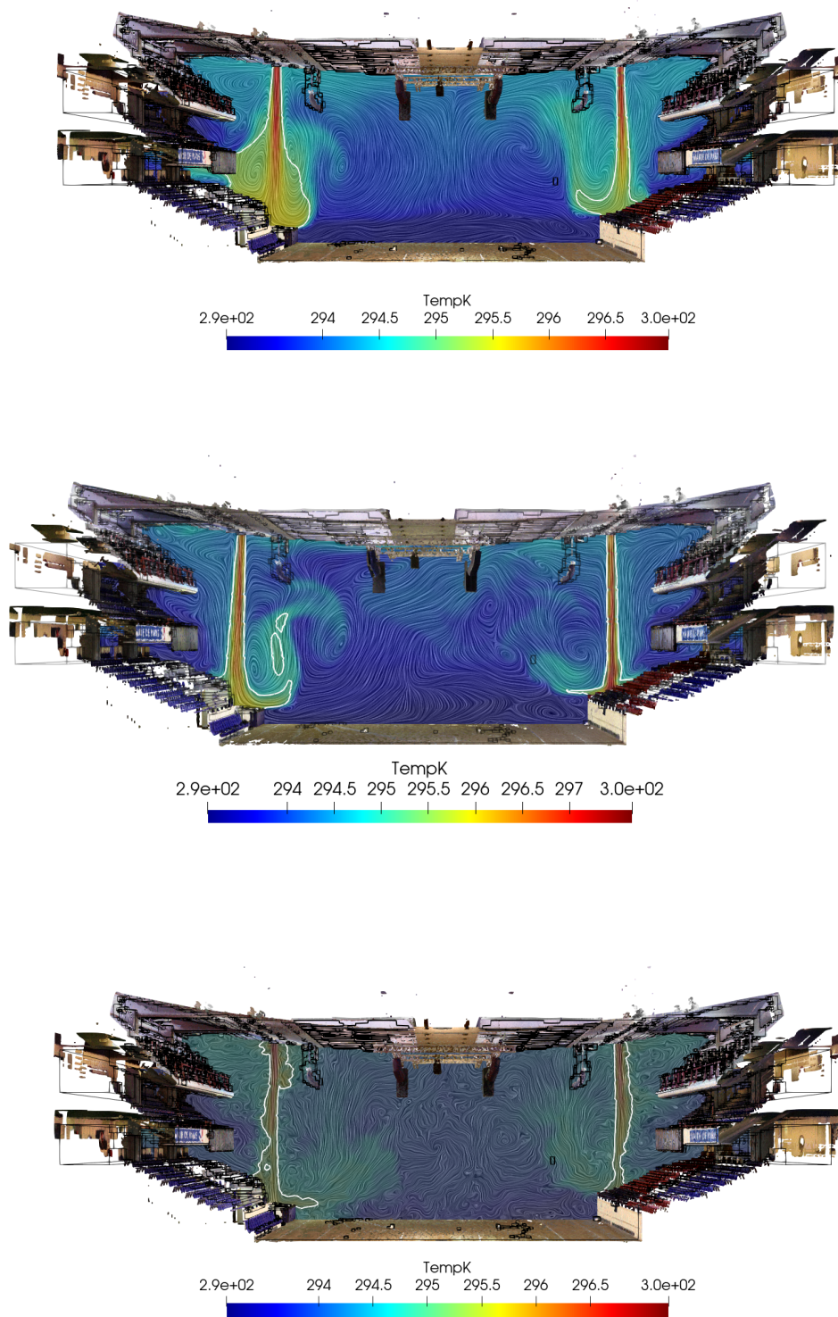
Figure 5.7.4: Slice of the temperature field (in colour) at the stadium mid width, with the isocontour T = 295 K at t = 300 s for the three turbulent simulations. (Top) k - \varepsilon . (Center) R_{ij} - \varepsilon . (Bottom) LES.
