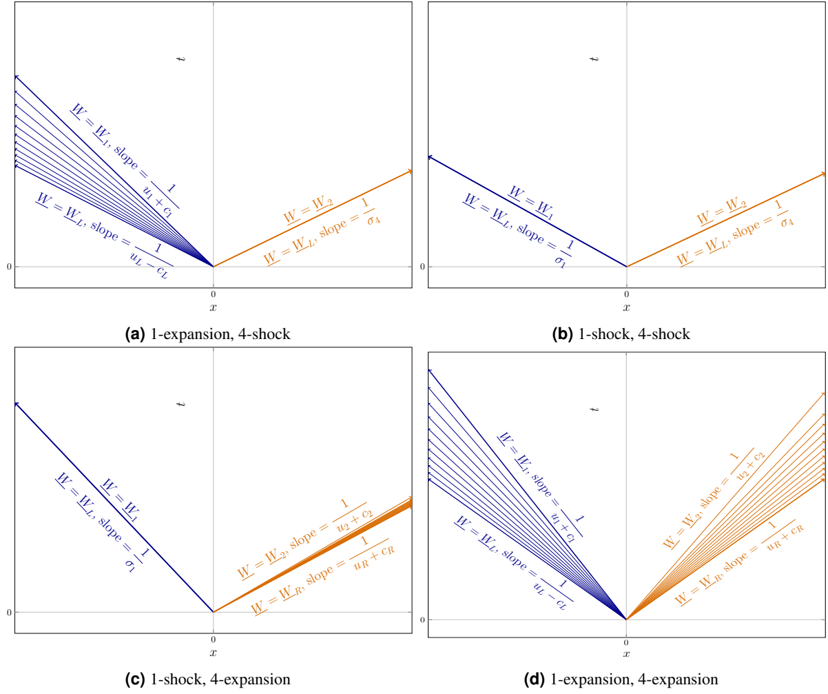
Figure 4.5.2: Sketch of the four possible cases for the one-dimensional Riemann problem.
