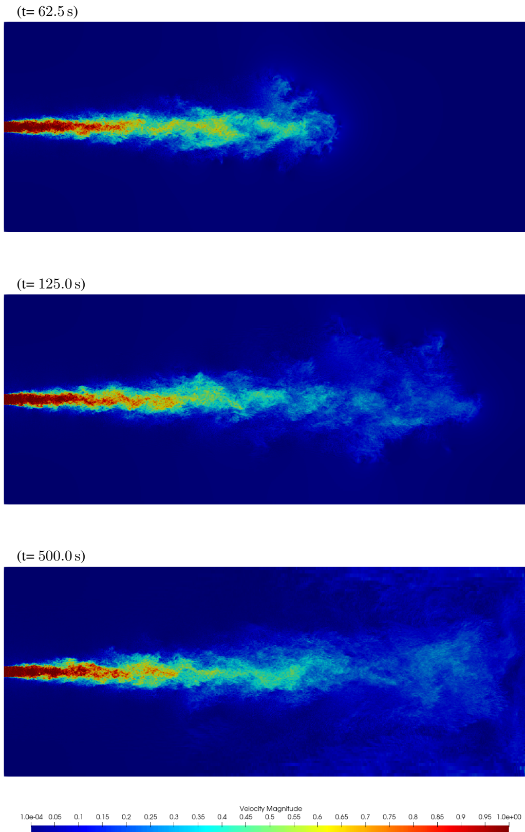
Figure 3.35: Velocity magnitude at different times for the most refined LES simulation.
