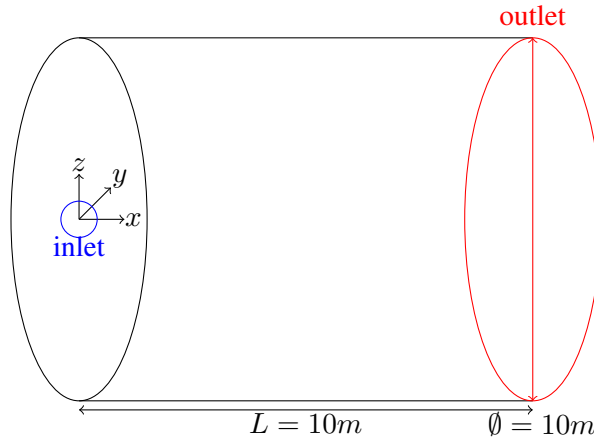
Figure 3.30: Setup sketch
