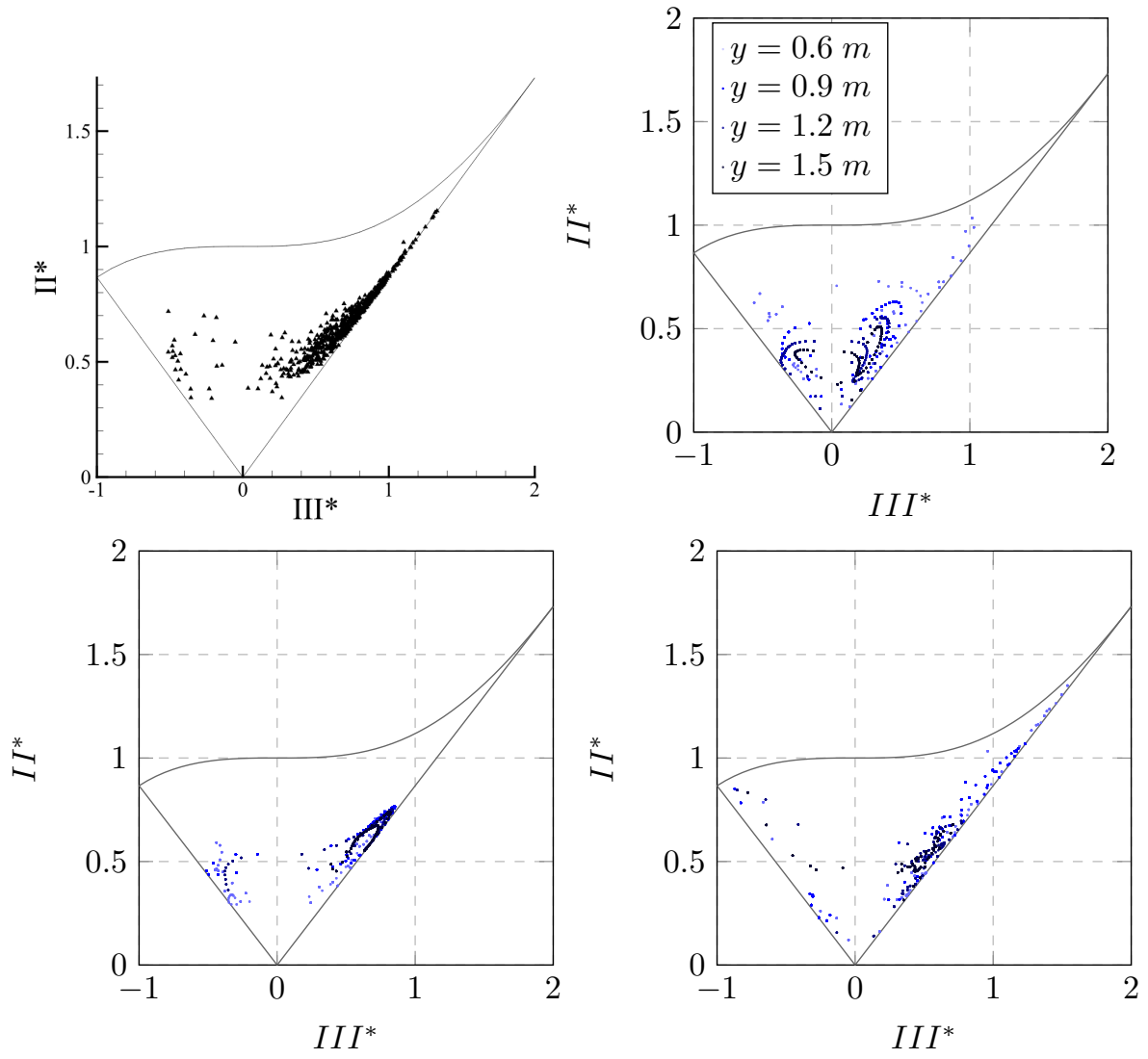
Figure 3.52: Lumley triangles for the isothermal jet case. Top left: experimental. Top right: k - \varepsilon . Bottom left: R_{ij} - \varepsilon . Bottom right: LES simulation.
