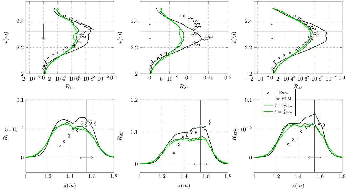
Figure 3.I.2: R_{ii} at y = 1.5 m for a simulation without SEM and two simulations with different eddy spatial length threshold values.
