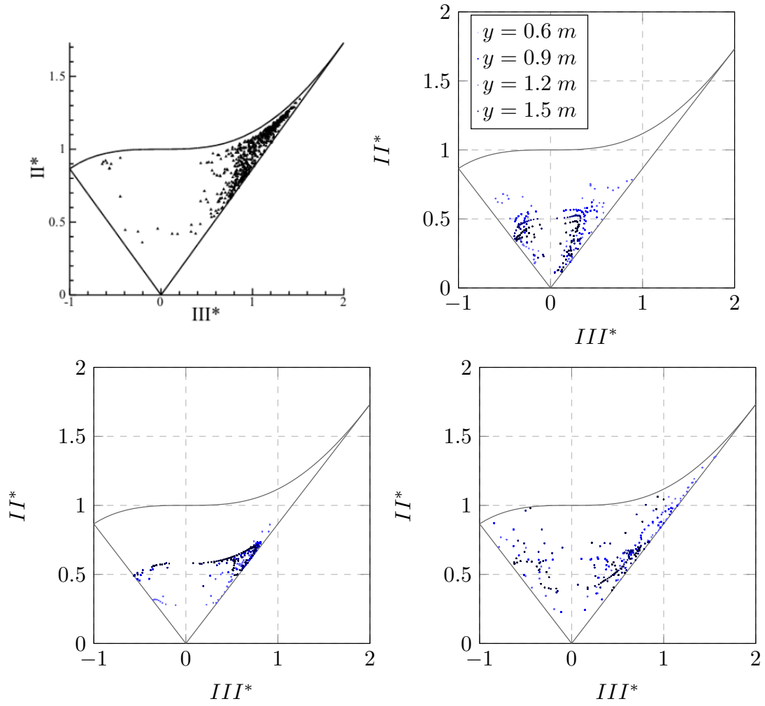
Figure 3.69: Lumley triangles for the cold jet case. (Top left) Experimental. (Top right) k - \varepsilon . (Bottom left) R_{ij} - \varepsilon . (Bottom right) LES simulation.
