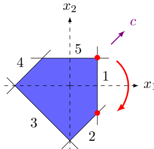
Figure 2.3: Illustration of a step of the simplex algorithm for a simple linear problem. We pivot from the basis \{1, 5\} to the basis \{1, 2\} .
