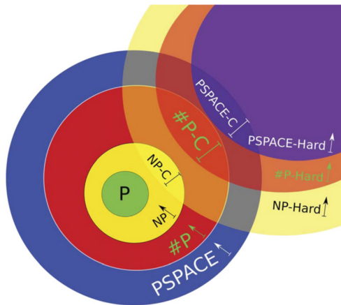
Figure 2.6: Different classes of complexity. The figure is borrowed from [IJC15].
