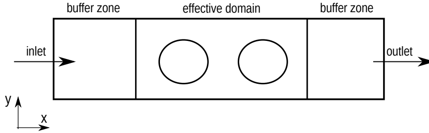
FIGURE 6.5 – Flow through a square array of cylinders. The array is modeled as a two dimensional problem and two cylinders (as considered in the references [9, 12]) are considered in the direction of the flow.
