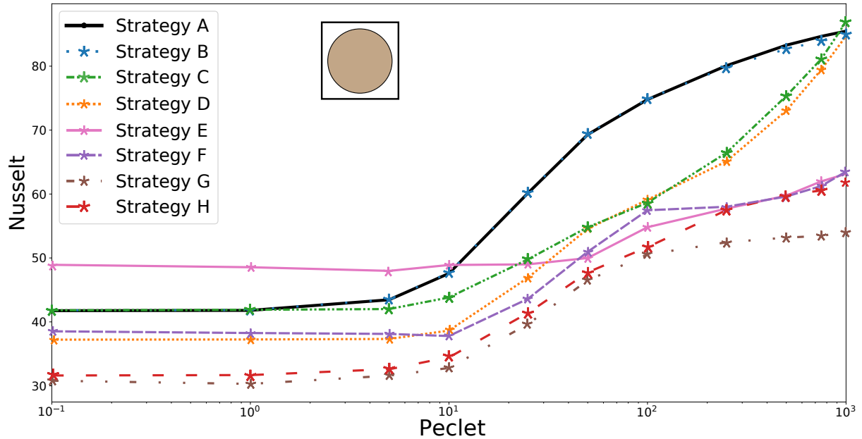
FIGURE 7.4 – Nusselt vs Peclet numbers for the test case (a) (Fig. 7.3) with porosity \epsilon = 0.38 . Strategies A, B, C, D, E, F, G, and H are adopted. Strategies A and B give the same predictions. Strategies D, E, F, G, and H lead to completely wrong results and are discarded. Strategy C gives good predictions (relative error lower than 5% for Pe < 10 ).
