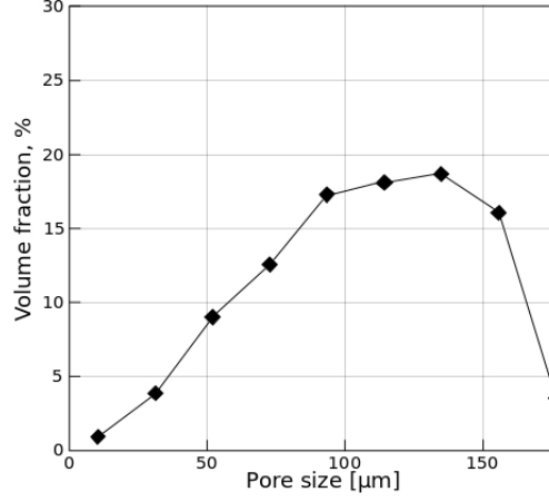
FIGURE 5.10 – Granulometry analysis done in Geodict [9]. The average pore-size in the through-thickness direction for the domain can be estimated to be equal to \ell_{\text{avg}} = 135 \mu\text{m} .
