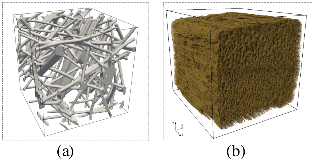
FIGURE 2.11 – High-resolution 3D tomography images considering for the determination of the effective properties. The Calcarb domain (a) is analyzed in Chapters 5, 6, and 7. The hard-wood match domain (b) is considered in Chapter 8.
