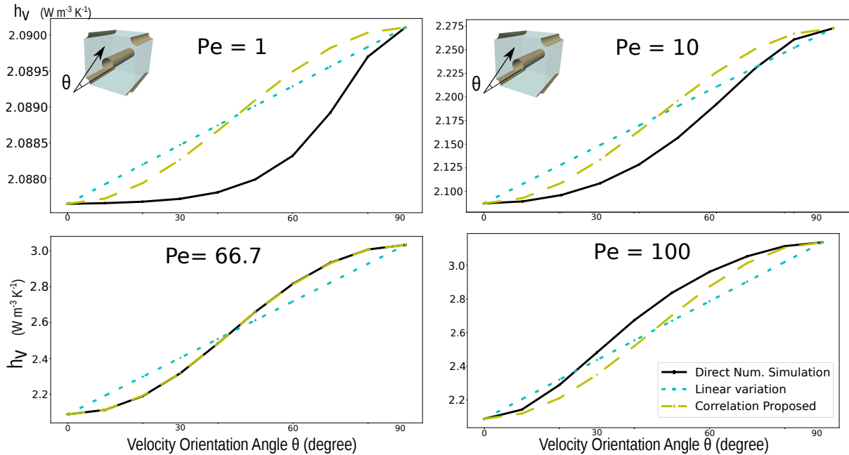
FIGURE 2.15 – Estimation of the anisotropy effects for the 2D periodic array of 5-cylinders case. A constant porosity \epsilon = 0.5 and different Peclet numbers are considered. The volumetric heat transfer tensor captures the shape of the anisotropic behaviour, but not its amplitude.
