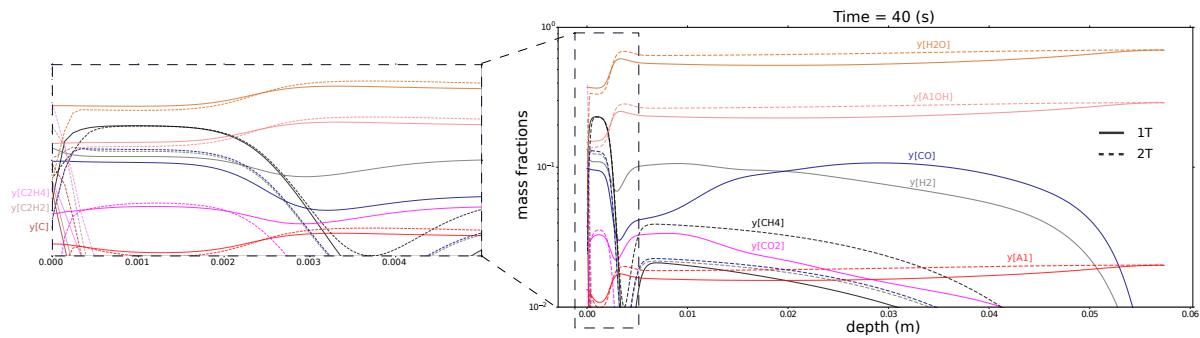
FIGURE 3.3 – Stardust case. Species distribution within the material at time t = 40 s. At the left: a zoom of the mass fractions near the surface with the external environment.
