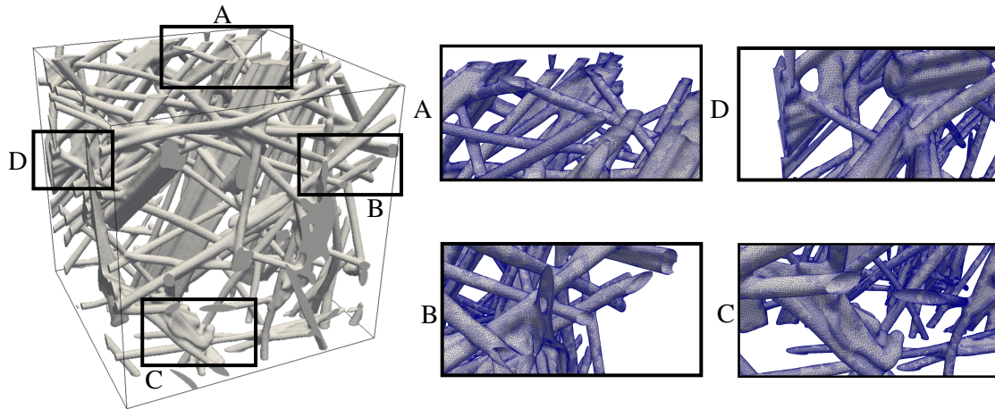
FIGURE 7.9 – On the left-hand side, volume rendering of the CMT of Calcarb. The dataset has a resolution of 200 \times 200 \times 200 voxels, with a voxel size of 2.6 \mu\text{g}m ; on the right-hand side, some details of the meshed geometry. The mesh accounts about 23 million cells.
