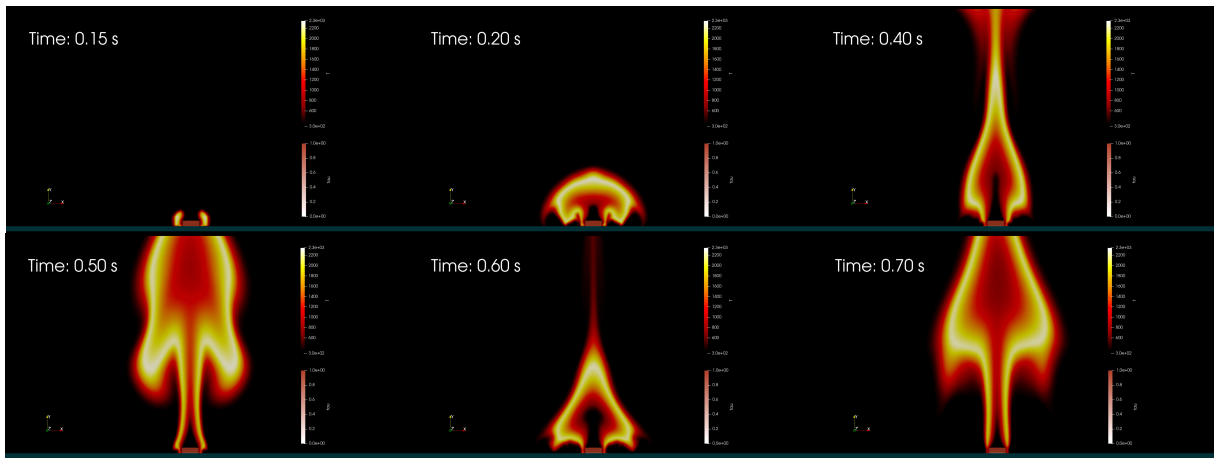
FIGURE 4.7 – Starting of the fire. Six different snapshots to represent the initial evolution of the fire. At time t = 0.15 s two sparks are generated on the side of the wood log to trigger the combustion. A fire is generated and start propagating in the domain. By comparing the time t = 0.50 s with the time t = 0.70 s it is possible to observe a periodic behaviour of the flame, the puffing effect.
