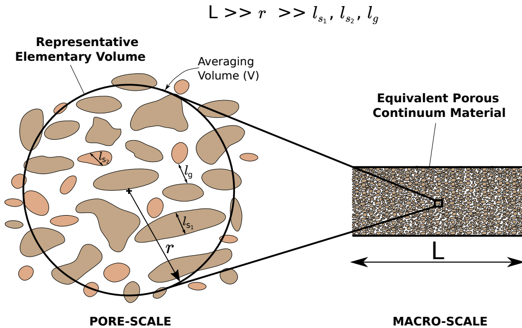
FIGURE 2.2 – Generic concept of the upscaling process. The process relies on the hypotheses of scale separation ( L \gg r \gg l_{s_1}, l_{s_2}, l_g ) and the existence of a REV where the small scale variations are smoothed.
