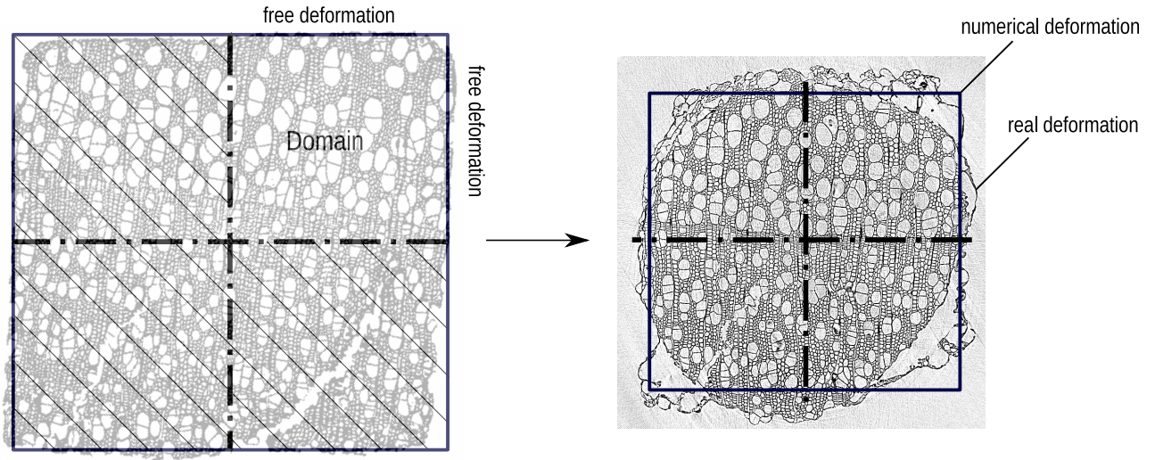
FIGURE 2.12 – Pyro-mechanical deformation of a 2D slice of domain (b) in the xy plane. The resulting numerical deformation is compared with the actual deformation undergone experimentally by the same cross section after a complete pyrolysis.
