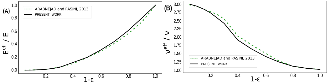
FIGURE 8.6 – Comparison of the effective elastic properties as a function of the solid fraction ( 1 - \epsilon ). The whole porosity range is considered. On the left (A), the behaviour of the effective Young modulus, normalized with the micro-scale value, is reported; on the right (B), the behaviour of the effective Poisson ratio, normalized with the micro-scale value, is showed. Comparison data are taken from the literature [4].
