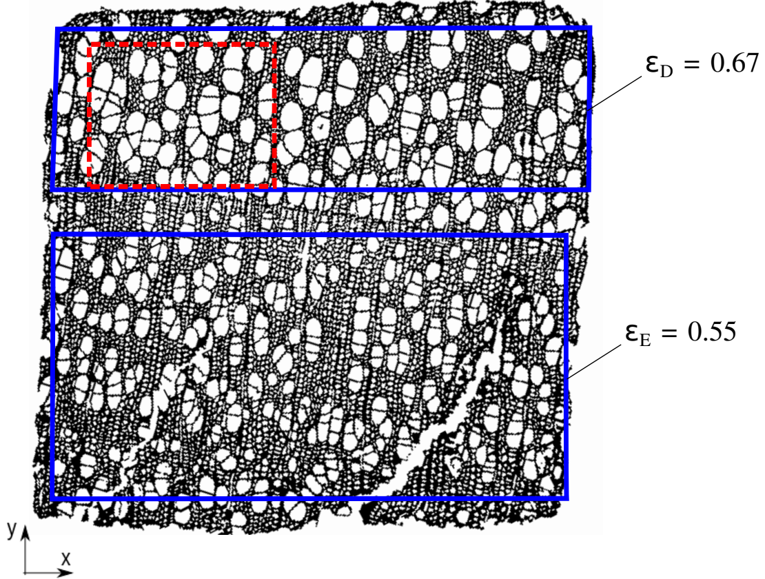
FIGURE 8.8 – Slice of the virgin wood sample (Fig. 8.1) in the transversal ( xy ) plane. The geometry shows two different regions featuring two different porosity values. In the red dashed domain, the two-step approach is tested. In the two blue continuous domains, the homogenization techniques are applied.
