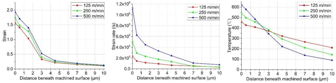
Fig. 74: The curve of plastic strain, strain rate and temperature distribution along the path in Fig. 73.
