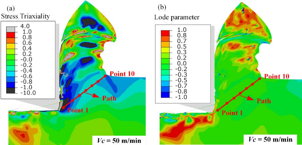
Fig. 45: Distribution of (a) stress triaxiality and (b) Lode parameter, obtained using LAG model for a cutting speed of 50 m/min.
