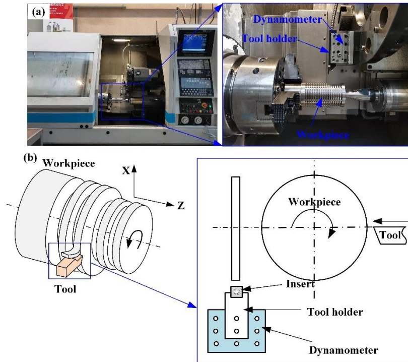
Fig. 96: Experimental tests using CNC lathe machine: (a) experimental setup, and (b) schematic representation of orthogonal cutting configuration.
