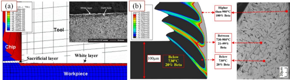
Fig. 13 Simulated phase volume fraction to predict the white layer formation in machined surface[76] and (b) Estimation of beta volume fraction in chip segmentation by SCM-based flow stress model [81].
