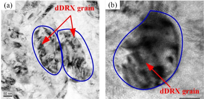
Fig. 79: TEM images of dDRX grains characteristics in machined subsurface in “Nano grains” layer of machined subsurface at cutting speed of 250 m/min.
