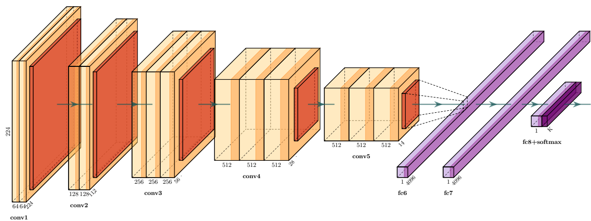
(a) VGG16
