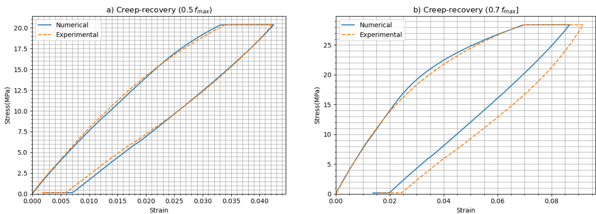
Figure 3.27: Calibration results for creep-recovery tests at RH80 under different loading levels: a) 50% of F_{\max} , b) 70% of F_{\max} .
