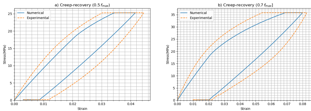
Figure 3.43: Calibration results for I_1 - J_2 -based model under creep-recovery tests at RH50 under different loading levels: a) 50% of F_{max} , b) 70% of F_{max} .
