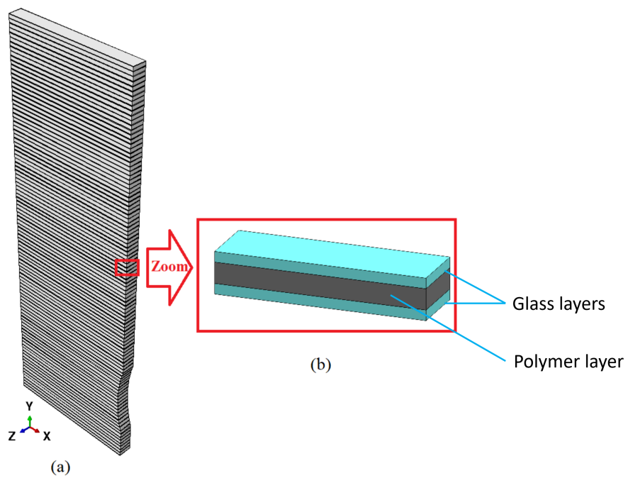
Figure 5.9: a) Multi-layered unilateral structure; b) zoom view and configuration of each RVE. The element type is the coupled temperature-displacement brick element (C3D8T)
