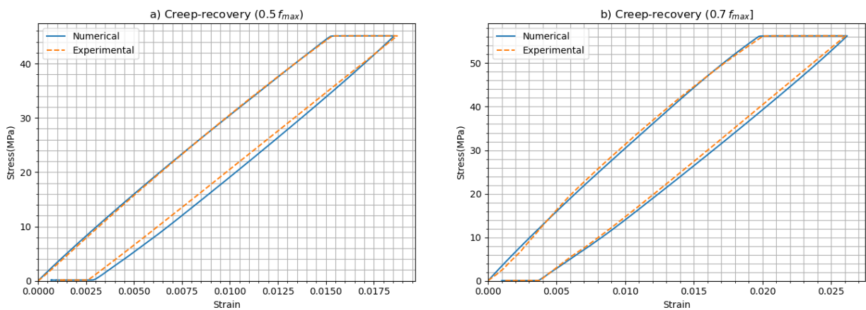
Figure 3.15: Calibration results for creep-recovery tests at RH0 under different loading levels: a) 50% of F_{\max} , b) 70% of F_{\max} .
