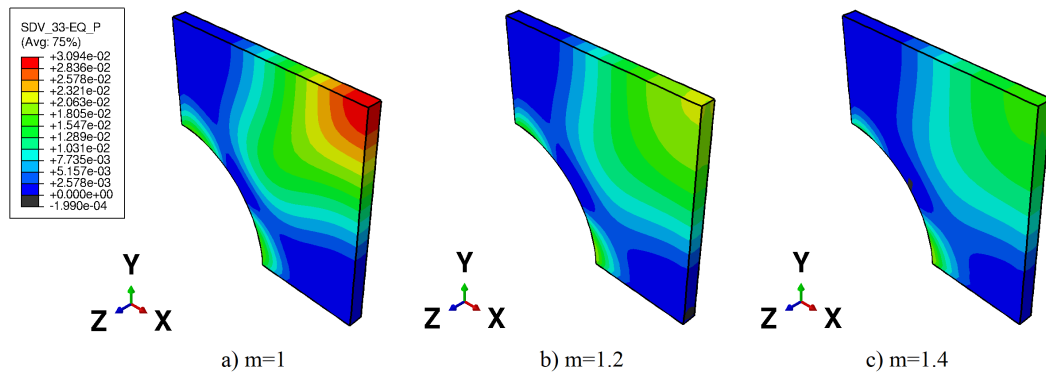
Figure 2.12: 3D maps of hardening state variable for 1/4 plate with a hole subjected to the multi-axial loading when a) m = 1 , b) m = 1.2 , and c) m = 1.4 .
