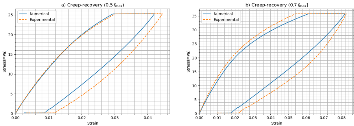
Figure 3.21: Calibration results for creep-recovery tests at RH50 under different loading levels: a) 50% of F_{\max} , b) 70% of F_{\max} .
