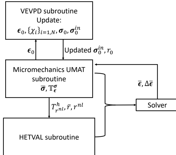
Figure 5.7: Flowchart of the numerical implementation in ABAQUS FE software for a composite structure. It should be mentioned that the HETVAL subroutine only needs T_h^{r^{nl}} , as the associated nonlocal tangent operator.
