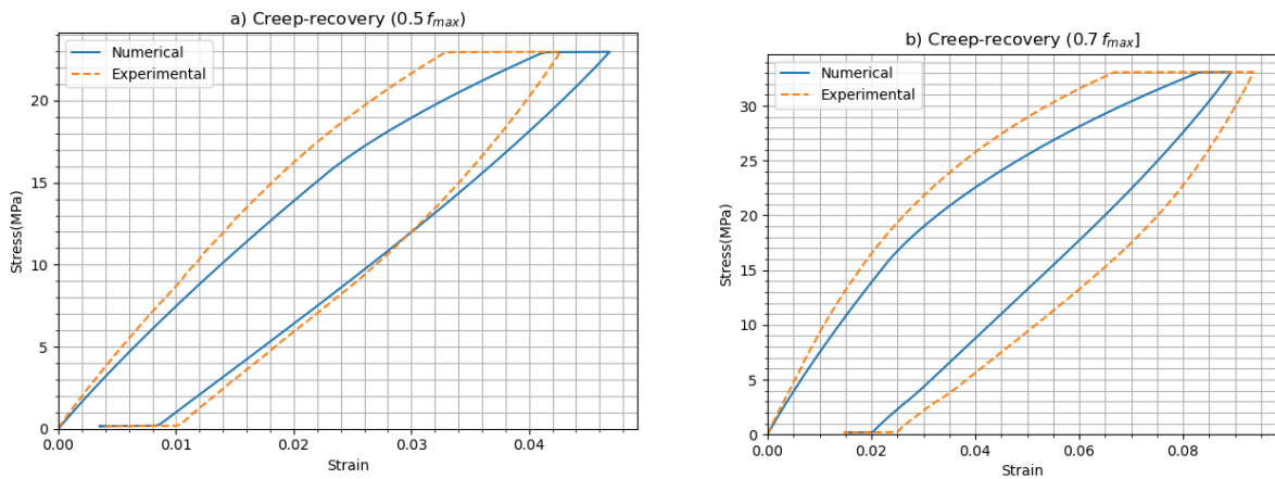
Figure 3.47: Calibration results for I_1 - J_2 -based model under creep-recovery tests at RH65 under different loading levels: a) 50% of F_{\max} , b) 70% of F_{\max} .
