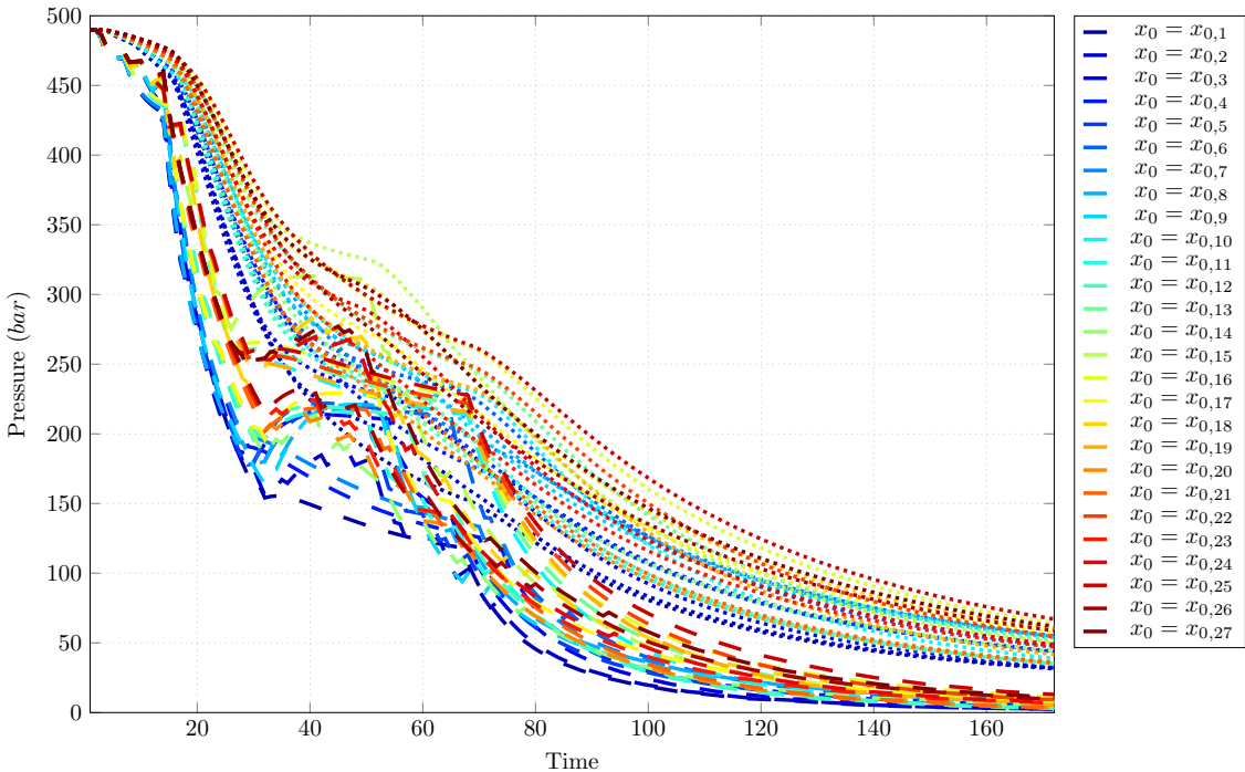
FIGURE 6.4: Evolution over time of the pressure when applying the optimal policy for all the possible initial states as listed in Equation (6.6). The pressures in the first tank are represented by the colored dashed curves, while the pressures in the second tank are represented by the colored dotted curves. Each color represents a given initial state
