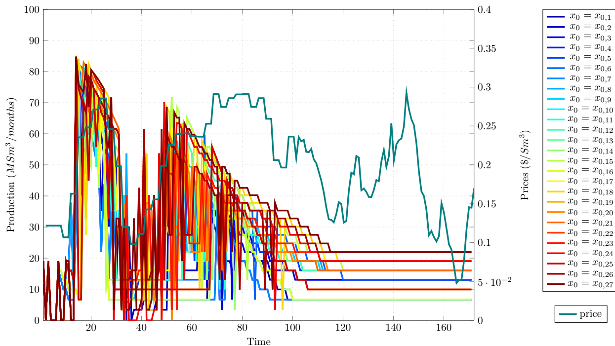
FIGURE 6.3: Evolution over time of the production (i.e. the control) when applying the optimal policy for all the possible initial states as listed in Equation (6.6), with the price curve in dark green. Each other color represents a given initial state
