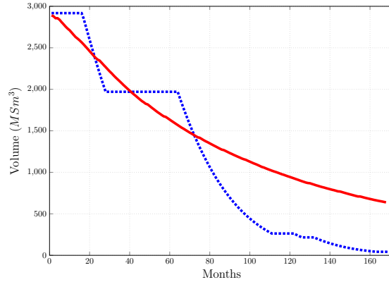
FIGURE 4.4: Evolution of the content of the reservoir in the one tank model. The dotted blue curve is the optimal (anticipative) trajectory of the amount of gas, while the red curve is the trajectory with the historical production
