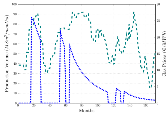
FIGURE 4.8: Trajectory of the optimal production in the two tanks model. The dotted blue curve is the optimal (anticipative) production, whereas the dashed green curve is the monthly gas price
