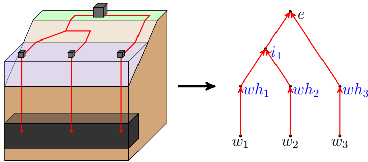
FIGURE 3.1: Representing a production network as a graph
