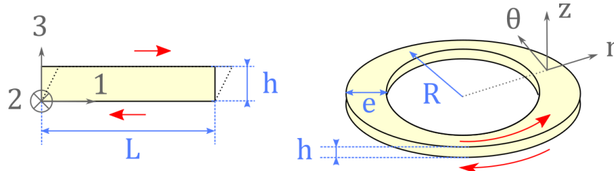
Figure 15: Space conventions for SLJ, TAST and ARCAN (left), and napkin ring (right). The red arrows symbolize the shear loading induced in the joint during sollicitation
