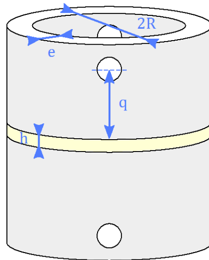
Figure 14: Napkin ring geometry
