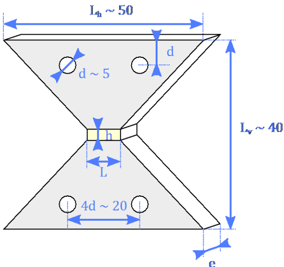
Figure 13: ARCAN geometry
