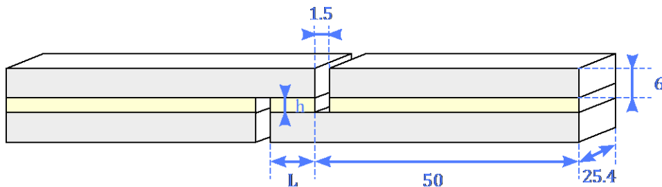
Figure 12: Thick Adherent Shear Test (TAST) geometry
