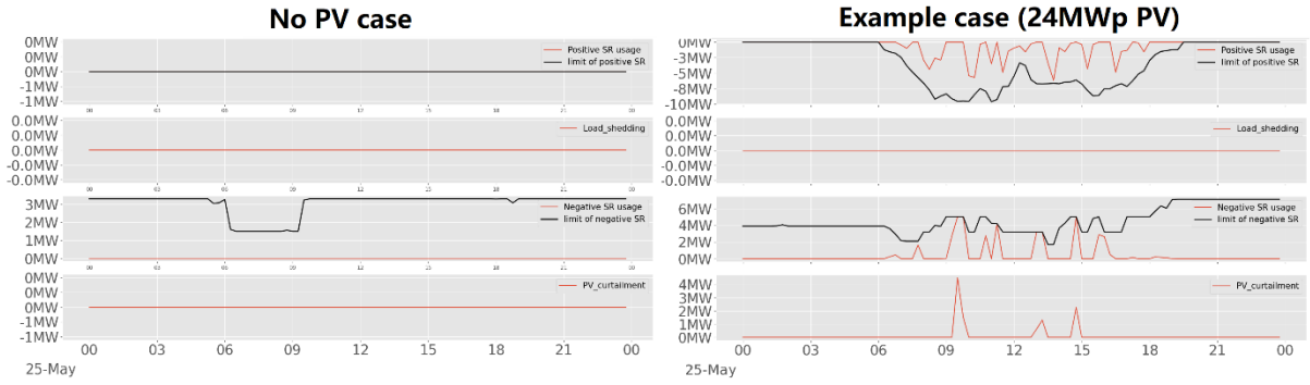
Figure 4.17 Detail of real data evaluation phase of no PV case
