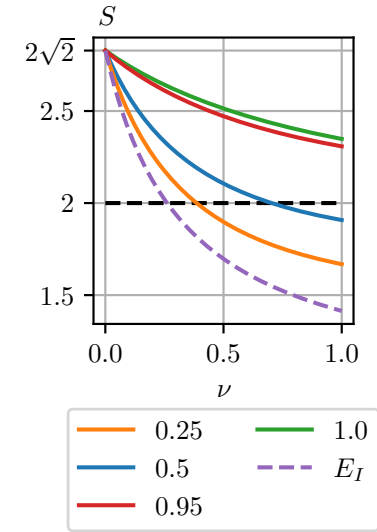
Figure 2.11: Bell parameter as a function of the population \nu , using the correlator E_{\text{III}} (2.49). The black dashed line represent the CHSH critical value. The lines are labelled with the quantum efficiency of the detectors. We also plotted (mauve dashed line) the result of the first approach for comparison. With the quantum efficiency of our detector ( \eta = 0.5 ) the Bell inequality is violated for \nu \lesssim 0.7 .
