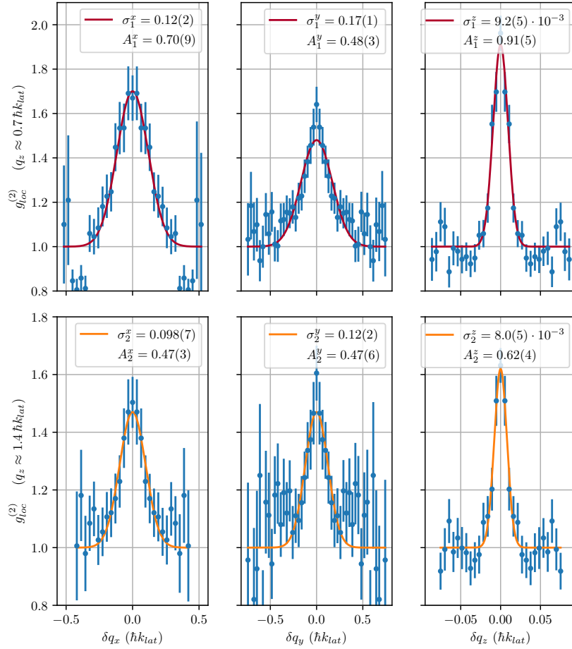
Figure 5.14: 1D local correlations as a function of the difference of quasi-momenta \delta q = q_1 - q_2 . Boxes (used to compute the correlations) are rectangular shaped, with widths \Delta v_i chosen such that they are smaller than the natural width of the modes in the probed direction, and roughly fitting the natural width of the modes in the transverse directions:
