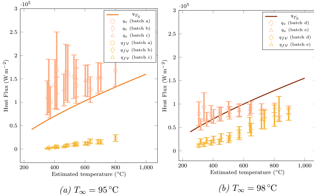
Figure 5.15: Comparison of experimental heat fluxes from the cooling rate estimation q_{T_S} , the vapour film thickness q_e and the vaporisation q_{fV} . q_e overestimates the heat fluxes for T_\infty = 95^\circ\text{C} and at lower overheating for T_\infty = 98^\circ\text{C} . The energy budget to vaporise the liquid q_{fV} is negligible for the T_\infty = 95^\circ\text{C} .
