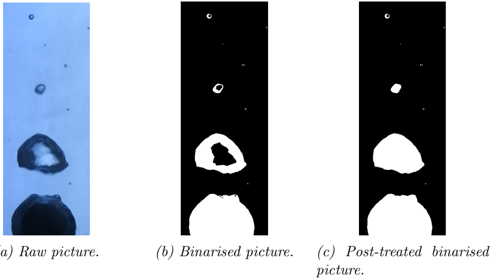
Figure 5.5: Example of the binarisation of an experimental picture from high speed camera. The liquid phase is identified with black pixels whereas the vapour and solid phases are in white. Reflection and refraction effects lead to misidentification of the vapour phase at the centers of bubbles that can be corrected with a filling function.
