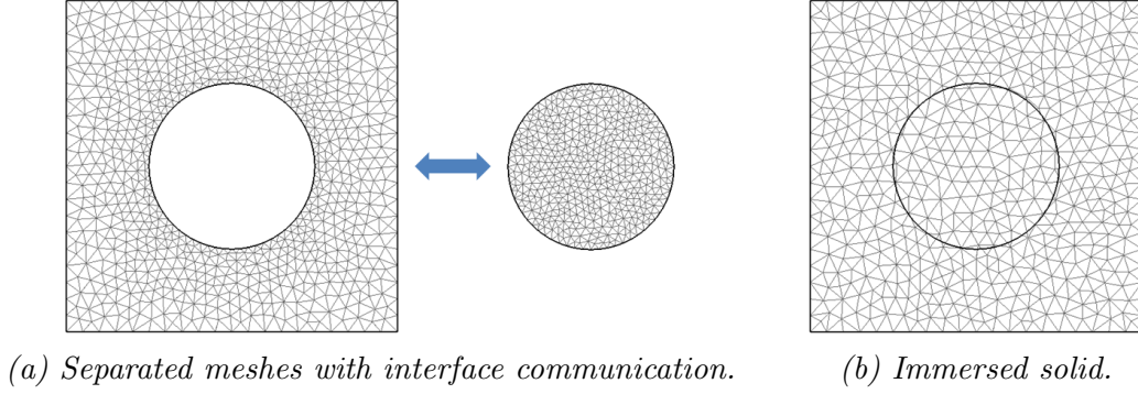
Figure 1.20: Example of separated and immersed domains.
