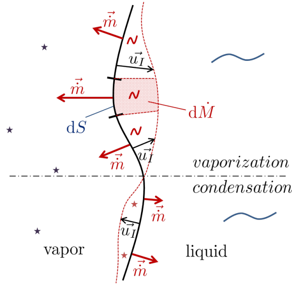
Figure 2.1: Schematic representation of the mass transfer rate vector. For vaporisation, the vector point towards the vapour. For condensation, it points towards the liquid.
