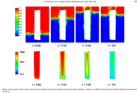
Figure 1.21: Simulation of the quench of a bar. The interface is not tracked but averaged quantities are considered. Correlations are used to estimate heat fluxes. (from [13]).
