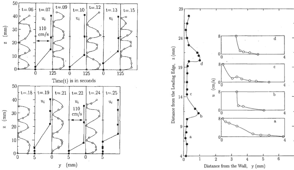
(a) Wave profile and phase velocity over time for \Delta T_w = 200 K and \Delta T_\infty = 1.5 K. (b) Wave profile and tangent liquid velocity profiles for \Delta T_w = 207 K and \Delta T_\infty = 6.7 K
