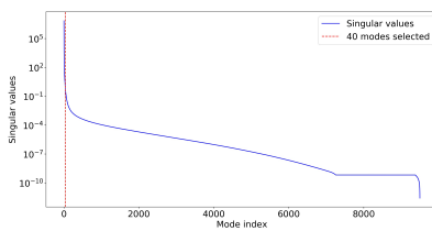
(a) POD pt displacement
