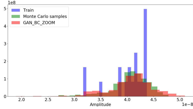
Figure 4.7: Histogram of maximum amplitude prediction
