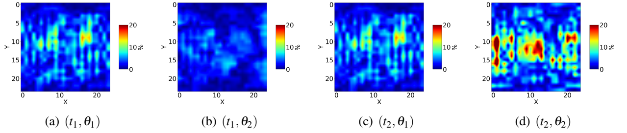
Figure 3.13: CNN_t error on S for displacement
