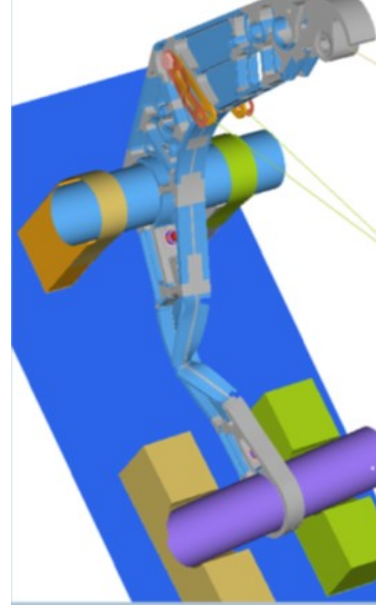
(b) Spreader stress simulation
