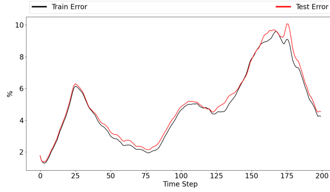
Figure 6.14: Regression error
