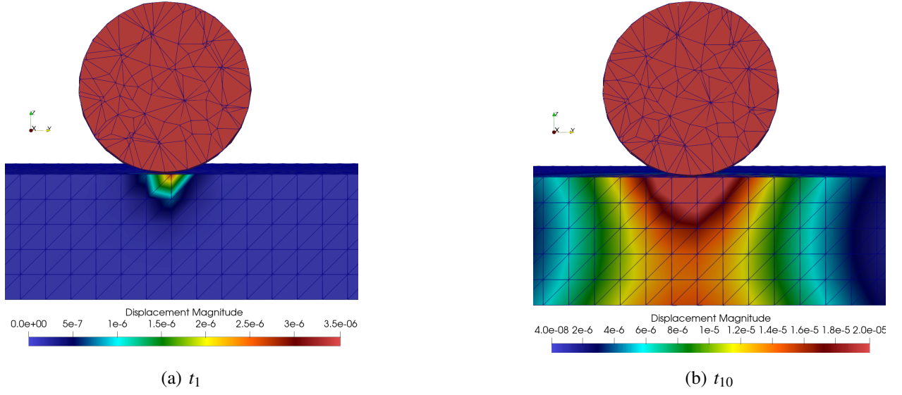
Figure 6.2: Cut-away view of the impact zone
