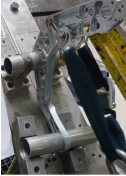
(a) Spreader stress experiment
