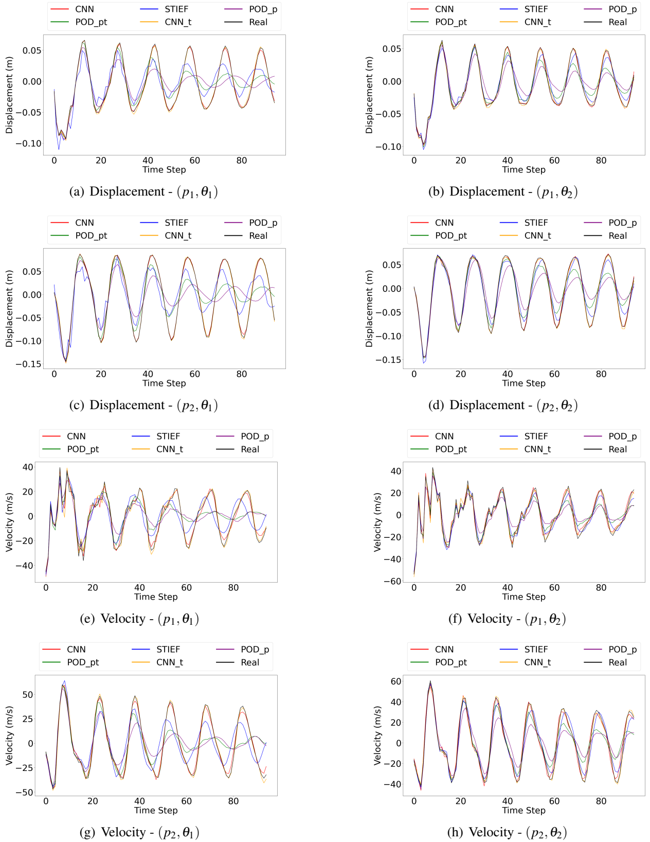
Figure 3.8: Models prediction on p_1 and p_2
