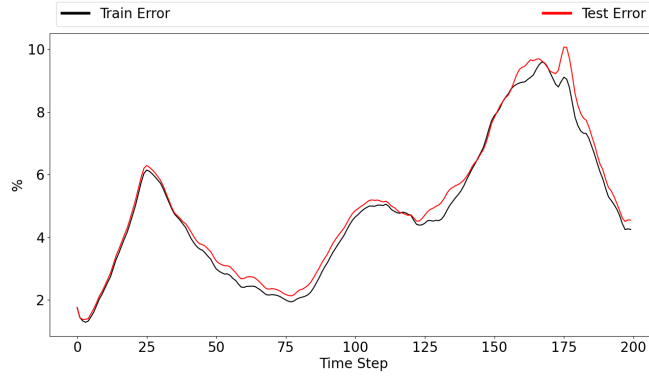
Figure 6.14: Regression error
