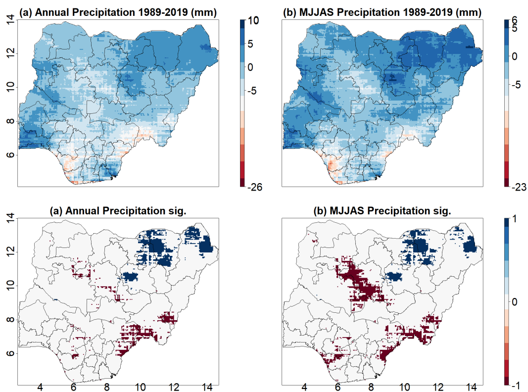
Figure C.6: Long-term trends of climate indicators - 1989-2019 long-term period
