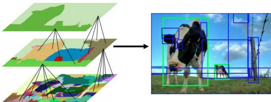
Figure 3.28: Selective Search iterative algorithm 15
