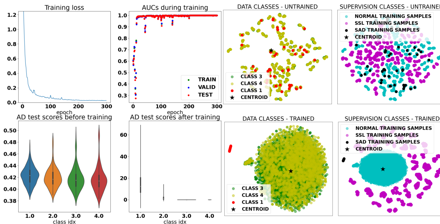
Figure 3.10: Left - Training metrics of a successful run where normal samples are concentrated around their average initial projection, and SAD and SSL samples are pushed away thanks to a loss term using the inverse of the distance with respect to the normality latent centroid. This is one of the most successful setups in Table 3.10, and one of the easiest AD experiments since the two classes defining normality here are class 3 (four blades are responsible for the modulation pattern around the central Doppler shift) and class 4 (six blades are responsible for the modulation pattern around the central Doppler shift), meaning the separation with the other classes deemed anomalous is actually a binary modulation complexity threshold. One of the contributions of the SAD and SSL supervisions can be observed on the evolution of AUCs during training: no AUC collapse can be seen during training, discarding the possibility of a latent distribution collapse during training. Experiments showed that large training batches contributed to stable AUCs growth. Spikes in the training loss match the drops in AUCs. Right - Latent distribution of the training samples visualized in 2D using t-SNE after projection by the untrained (top) and the trained neural network (bottom). One can notice that normal training samples from both normal classes are completely mixed up with the minority of SAD labeled anomalies from class 1 in red (one blade), semantically similar, whereas SSL samples which are rotated normal training samples are already gathered in their own latent subclusters. SAD labeled anomalies end up well separated after training.
