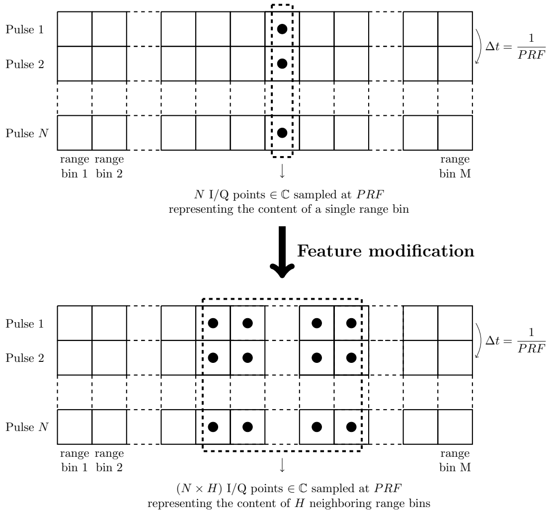
Figure 1.3: The proposed detections filter modifies the existing I/Q attribut of hits to integrate a neighborhood of range cells over the whole burst of pulses to provide the discrimination with additional information. In this figure the vertical axis describes the slow time of the sampling happening at PRF , i.e. between pulses, while the horizontal axis describes the fast time of the sampling happening at a much higher frequency and harbouring the range cells. The PRF is the sampling frequency that varies between hits, introducing a challenging physical diversity between input data points, the overall diversity also stemming from the varying number of pulses. The number of pulses here corresponds to N , the number of rows. Respecting the low-resolution constraint, we will consider N \in \llbracket 8, 32 \rrbracket , as these are typical values for Pulse-Burst radars (PBR) [167, p.188][133, p.470], which will be considered as equivalent to air surveillance PDRs in this thesis. The fast time, much higher, sampling frequency is considered to be constant across all hits and systems considered. An illustration of this diversity is proposed on Fig. 1.4. Top: original hit object I/Q feature (1D complex-valued vector) Bottom: new hit object I/Q feature (2D complex-valued matrix).
