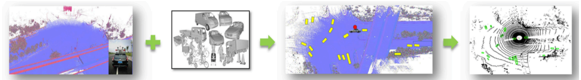
Figure 5.2: In [Fang et al. 2020], first the scene is modeled, then CAD models of dynamic objects, such as vehicles, pedestrians and cyclists are added to generate a new scenario in which the LiDAR is simulated. Source [Fang et al. 2020]
