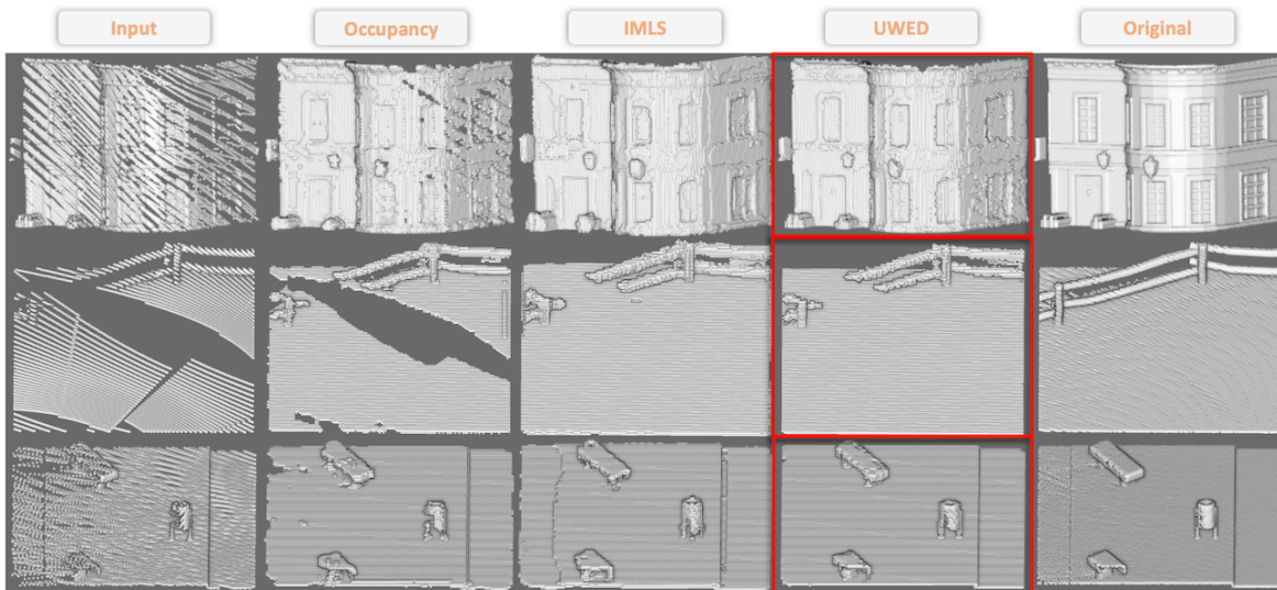
Figure 3.15: Scene completion inference of MinCompNet using Occupancy, IMLS, and our UWED function as input on the PC3D-CARLA test set (input has 10% of the original points) and predicting occupancy.
