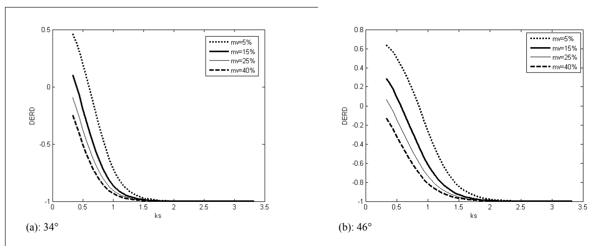
Fig. 13. Behaviour of the DERD from the IEM data as a function of the soil moisture and ks . F=5.3\text{GHz} , Exponential autocorrelation function, incidence angles = 34° and 46°.
