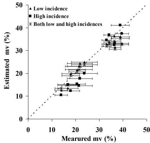
Fig. 4. Comparison between the estimated mv-values and those measured. The error bars on the measured soil moisture values correspond to one standard deviation.
