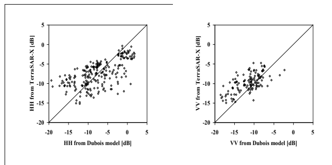
Fig. 3. \sigma_{HH}^{\circ} and \sigma_{VV}^{\circ} measured from TerraSAR-X images versus those simulated from Dubois model.
