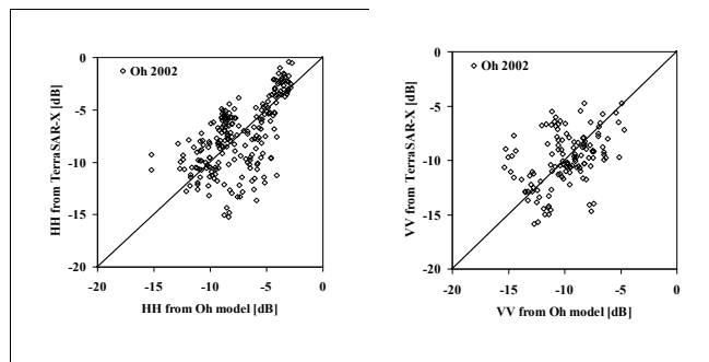
Fig. 2. \sigma_{HH}^{\circ} and \sigma_{VV}^{\circ} measured from TerraSAR-X images versus those simulated from 2002 Oh model.
