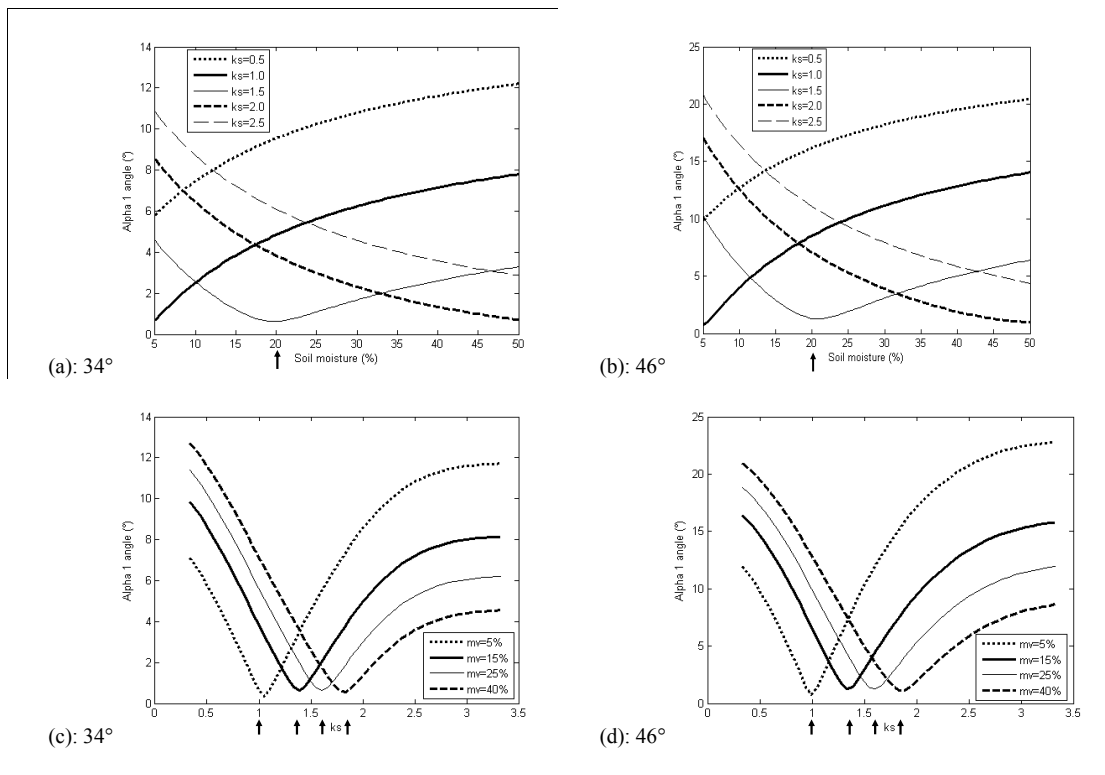
Fig. 5. Behaviour of \alpha_1 from the IEM data as a function of the soil moisture and ks . F=5.3\text{GHz} , Exponential autocorrelation function, incidence angles = 34^\circ and 46^\circ . The change of the polarimetric behaviour is indicated by arrows.
