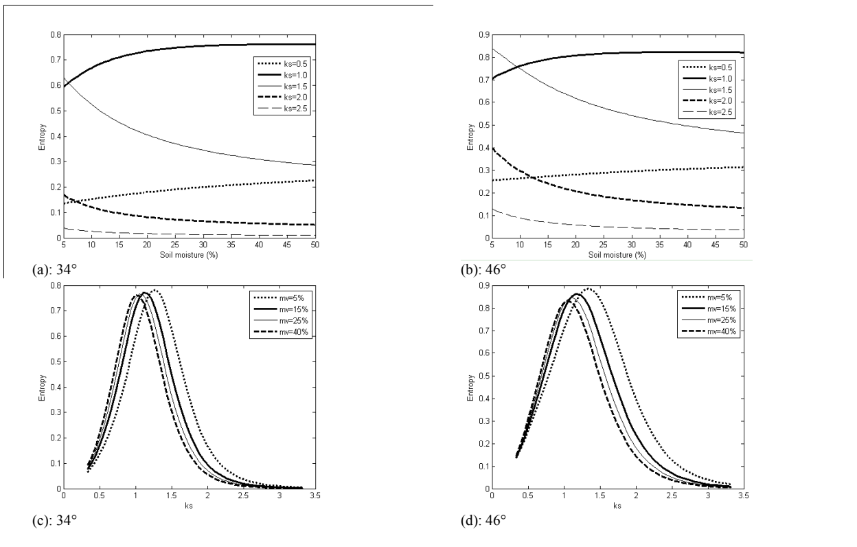
Fig. 7. Behaviour of entropy from the IEM data as a function of the soil moisture and ks. F=5.3\text{GHz} , Exponential autocorrelation function, incidence angles = 34° and 46°.
