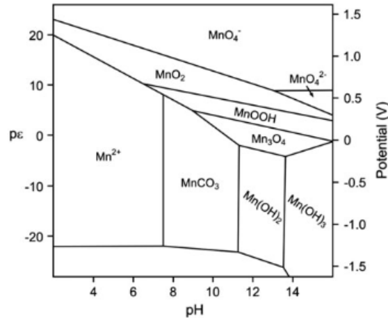
Figure 6 - Different forms of Manganese according to electron activity ( p\epsilon ), pH and redox-potential (Bruins et al., 2014).
