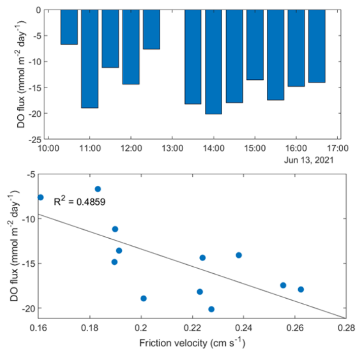
Figure 53 - A) turbulent benthic oxygen fluxes (eddy covariance) during the June 13 2021 campaign. B) Relation between oxygen fluxes and the friction velocity.
