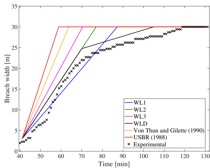
Figure 3.43: Comparison of computed breach widths with linear erosion equations.
