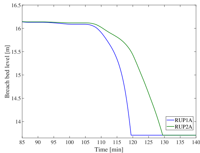
Figure 3.30: Comparison of computed bed level for different RUPRO model options and K_d = 60 \text{ (cm}^3/(\text{s Pa})\text{)} .
