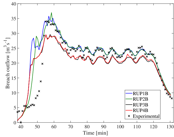
Figure 3.53: Comparison of computed breach discharge for different RUPRO model options for K_d = 80 \text{ (cm}^3/(\text{s Pa}) \text{)} (Case 2).
