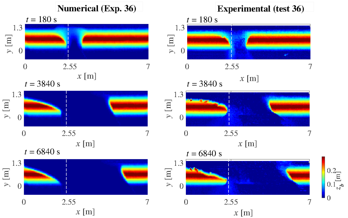
Figure 4.4: Simulated and measured 3D breach shapes for Test 36 (the dashed White lines indicate initial notch location).
