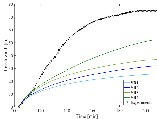
Figure 3.14: Measured and computed time-evolution of breach width with the Verheij and Van der Knaap (2003) law.
