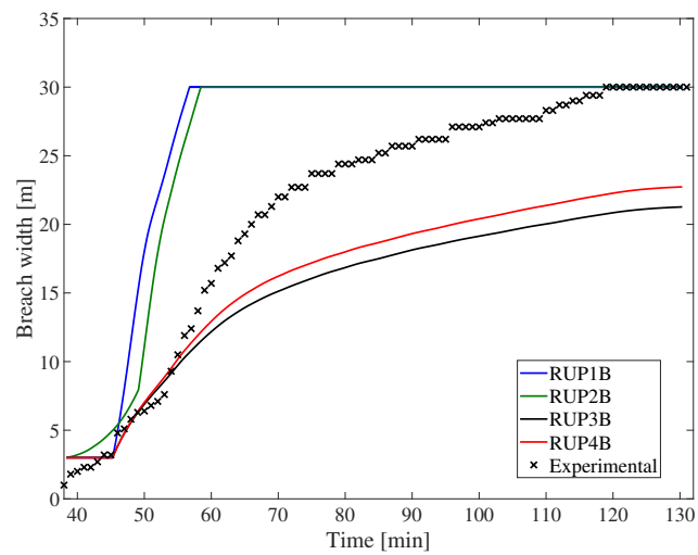
Figure 3.54: Comparison of computed breach width for different RUPRO model options for K_d = 80 \text{ (cm}^3/(\text{s Pa}) \text{)} (Case 2).
