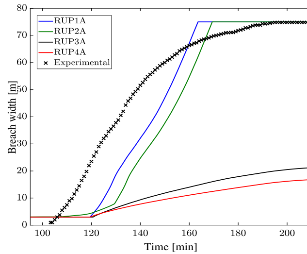
Figure 3.29: Comparison of computed breach width for different RUPRO model options and K_d = 60 \text{ (cm}^3/(\text{s Pa})\text{)} .
