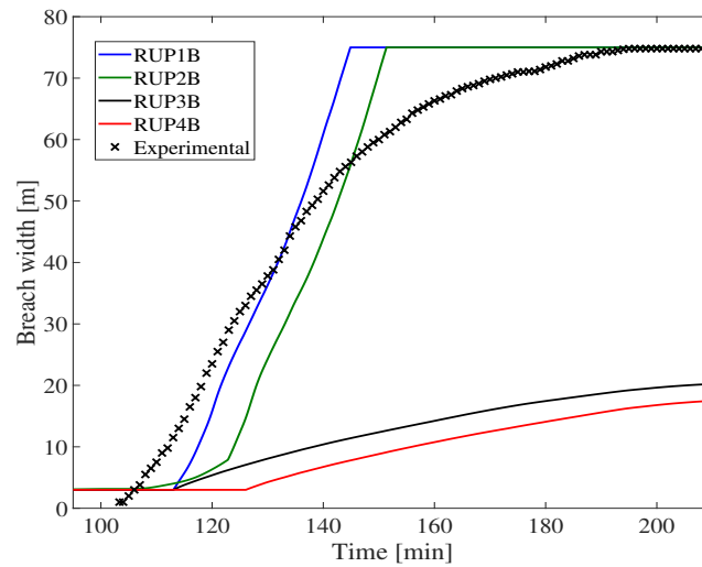
Figure 3.32: Comparison of computed breach width for different RUPRO model options and K_d = 80 \text{ (cm}^3/(\text{s Pa})\text{)} .
