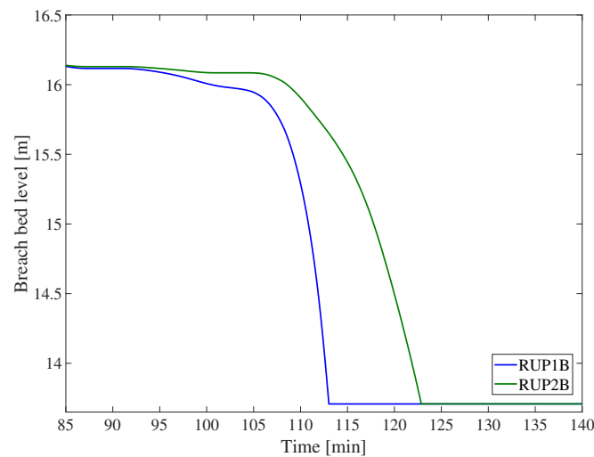
Figure 3.33: Comparison of computed bed level for different RUPRO model options and K_d = 80 \text{ (cm}^3/(\text{s Pa})\text{)} .
