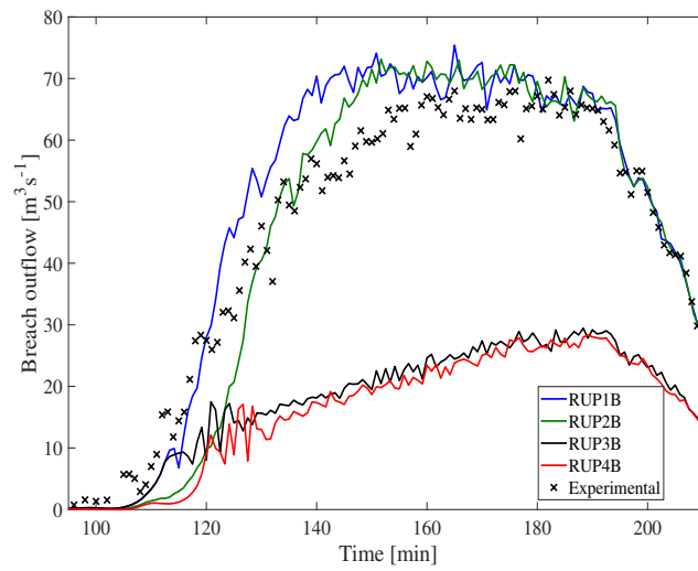
Figure 3.31: Comparison of computed breach discharge for different RUPRO model options and K_d = 80 \text{ (cm}^3/(\text{s Pa})\text{)} .
