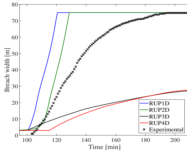
Figure 3.38: Comparison of computed breach width for different RUPRO model options and K_d = 120 \text{ (cm}^3/(\text{s Pa})\text{)} .
