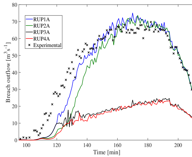
Figure 3.28: Comparison of computed breach discharge for different RUPRO model options and K_d = 60 \text{ (cm}^3/(\text{s Pa})\text{)} .
