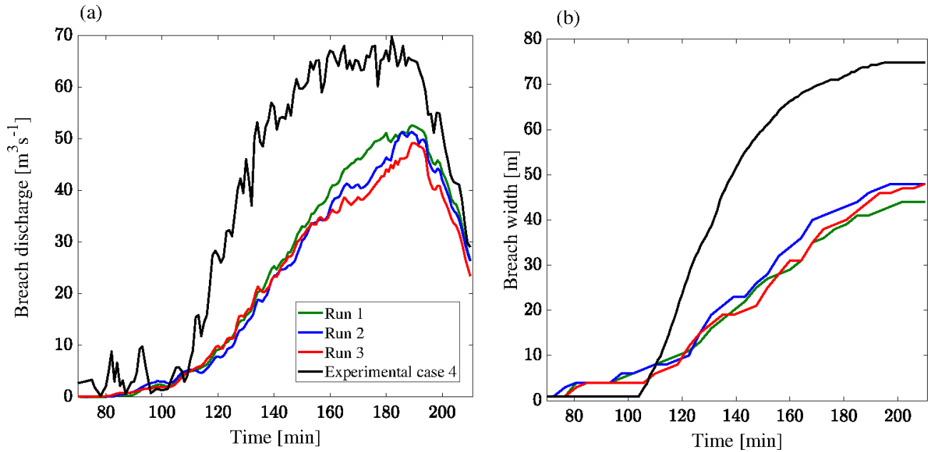
Figure 4.16: Comparison of Case 4 simulations with \alpha_y = 12 and different \alpha_x values : (a) breach discharge and (b) breach width at the crest level ( y = 89 m).
