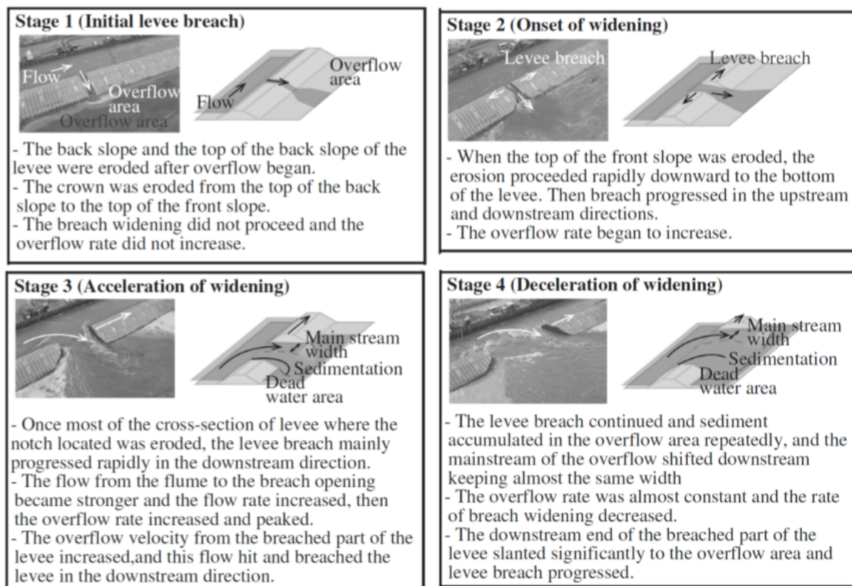
Figure 1.13: Levee breach stages description by Kakinuma and Shimizu (2014).
