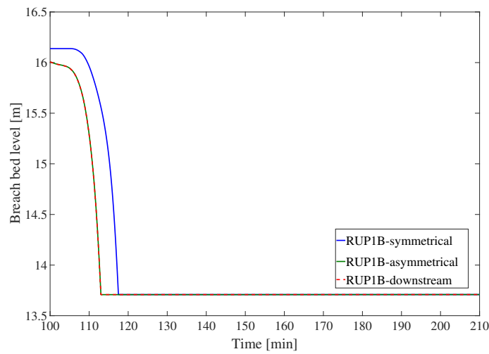
Figure 3.27: Influence of widening configuration on breach bed level of RUPRO model and K_d = 80 ( \text{cm}^3/(\text{s Pa}) ).
