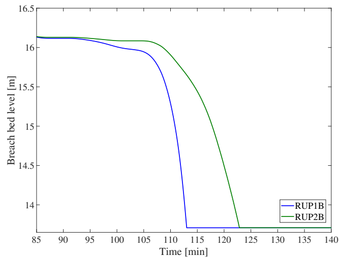
Figure 3.55: Comparison of computed breach bed level for different RUPRO model options for K_d = 80 \text{ (cm}^3/(\text{s Pa}) \text{)} (Case 2).
