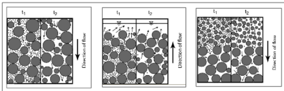
Figure 1.8: Illustration of suffusion (Riha et al. (2019)).
