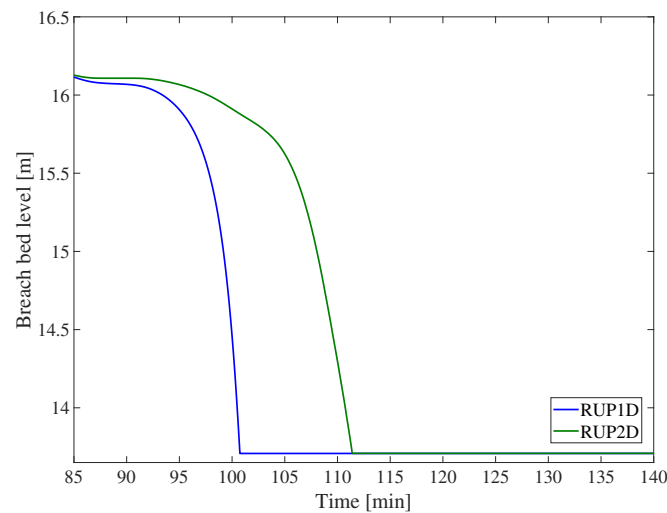
Figure 3.39: Comparison of computed breach bed level for different RUPRO model options and K_d = 120 \text{ (cm}^3/(\text{s Pa})\text{)} .
