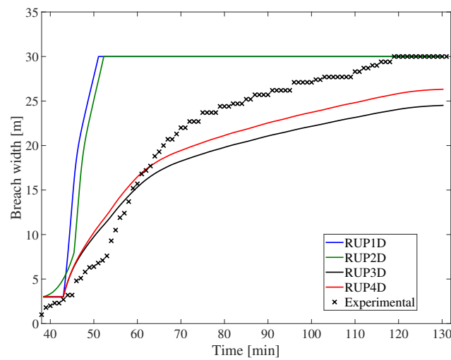
Figure 3.60: Comparison of computed breach width and bed level for different RUPRO model options for K_d = 120 \text{ (cm}^3\text{/s Pa)} .
