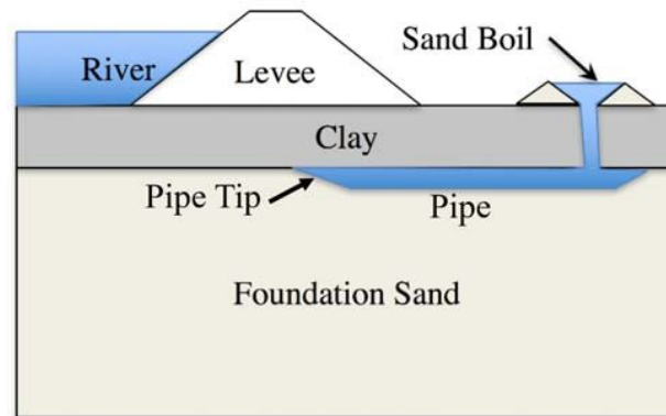
Figure 1.7: Illustration of backward erosion ( Orlando, Florida, 2019Montalvo-Bartolomei and Robbins Orlando, Florida, 2019 Orlando, Florida, 2019).
