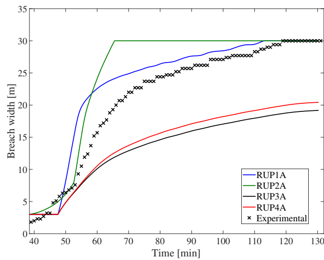
Figure 3.51: Comparison of computed breach width for different RUPRO model options for K_d = 60 \text{ (cm}^3\text{/s Pa)} (Case 2).
