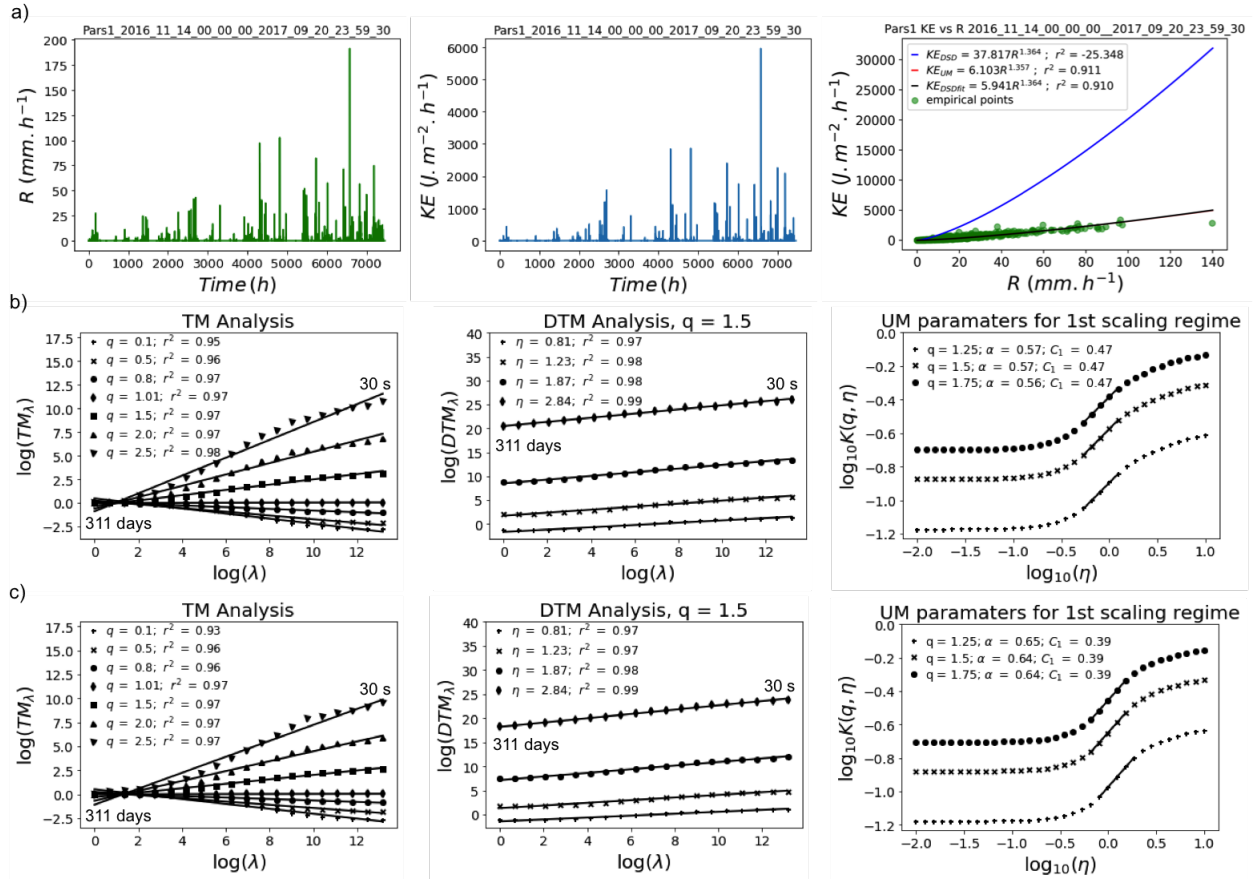
Figure 2.3: a) Time series of R , time series of KE , KE vs R graph b) and c) Multifractional analysis graphs with KE and R (log-log plot of Eq. 14 and Eq. 22 for TM and DTM analysis respectively and log-log plot of exponents in Eq. 22 for UM parameters) using the year based analysis, for Pars 1, for 2017
