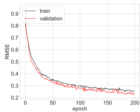
(n) Learning curves BPNN
