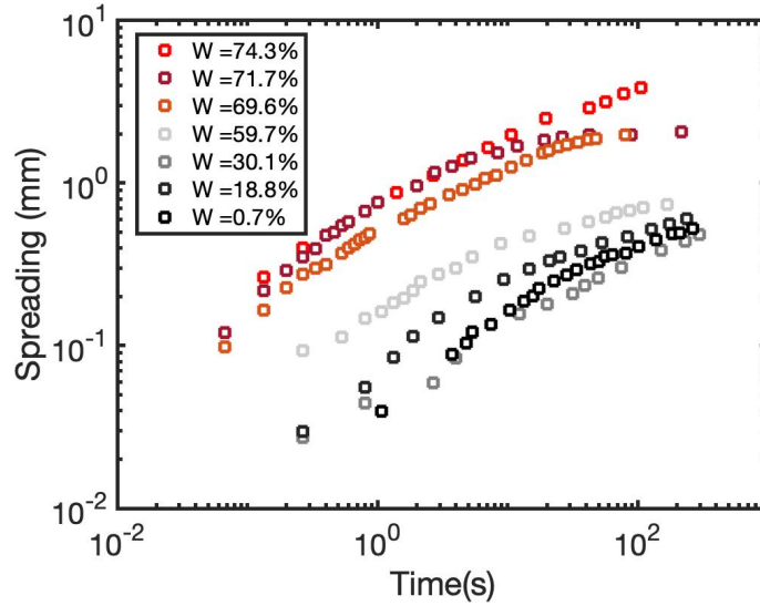
Figure 4.12: Spreading (increase of the diameter) of a water drop over a hydrogel surface at different water concentration ( C in %).
