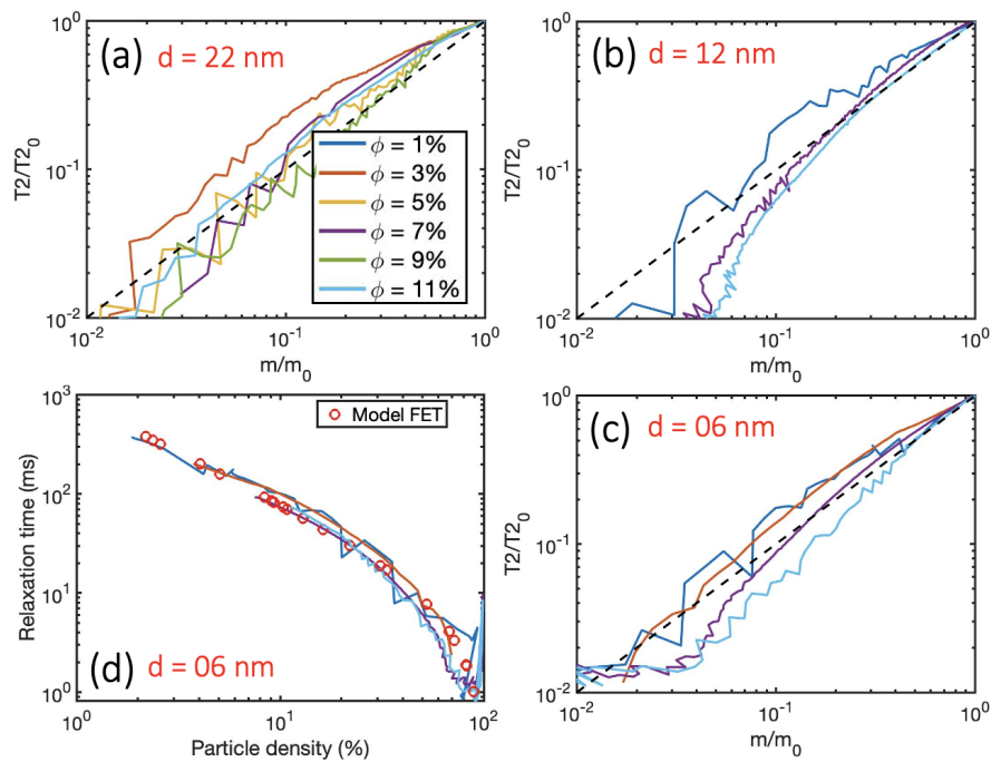
Figure 5.10: Representation of the normalize relaxation time according to the normalize water content at different particle densities for various bead size: (a) 22 nm, (b) 12 nm and (c) 6 nm. The dotted black lines have a slope of one. (d) Evolution of the representative relaxation time according to the particle density obtained from (red dots) the FET model (equation 5.3) (plain lines) from the water mass evolution.
