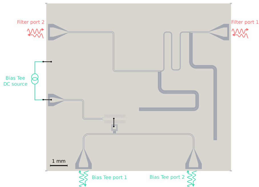
Figure 4.10: Graphic presentation of the chip used for testing the stop-band filter. It is based on the drawing file that was used to pattern the circuit with laser lithography. Blue represents silicon. Grey represents niobium. Bonds are signaled with black lines. This chip is intended for testing two distinct on-chip electromagnetic components. The top part of the chip is dedicated to testing stop-band filter: the red waves signal the two RF-ports. The bottom part is dedicated to testing on-chip bias tee: the green waves signals the two RF-ports, the green straight line represents the DC connection.
