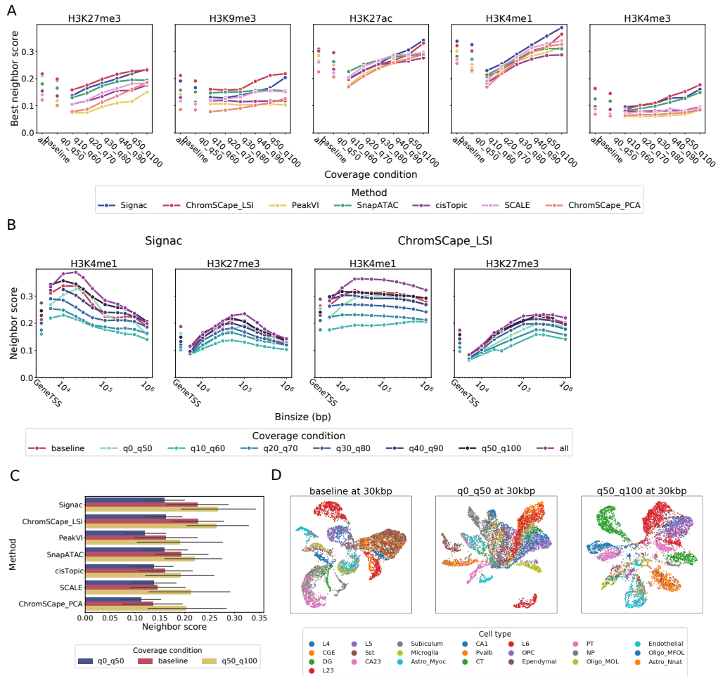
Figure 4.7: Study of the effect of cell coverage on the performances of the representations. The all condition contains all the cells as a reference, the baseline condition contains only 50% of the cells uniformly sampled at random, the other 6 conditions contain 50% of the cells, but are sorted by coverage. We order the cells by how much reads they contain and take all the cells from the bottom n\% up to n + 50\% in order to have the same amount of cells in all conditions. A Best performance across matrix construction, measured for all of the 7 methods, 5 marks of the mouse brain dataset and 8 coverage conditions. B . Performances of Signac and ChromSCape_LSI on H3K4me1 and H3K27me3 as a function of matrix construction. C . Average best performance of the 7 methods across all marks, for the lowest covered cells, random cells, and highest covered cells. D . UMAP projection of H3K4me1 at different coverage qualities, using ChromSCape_LSI across at 30kbp, colored by the labels of [71] obtained from the scRNA-seq co-assays.
