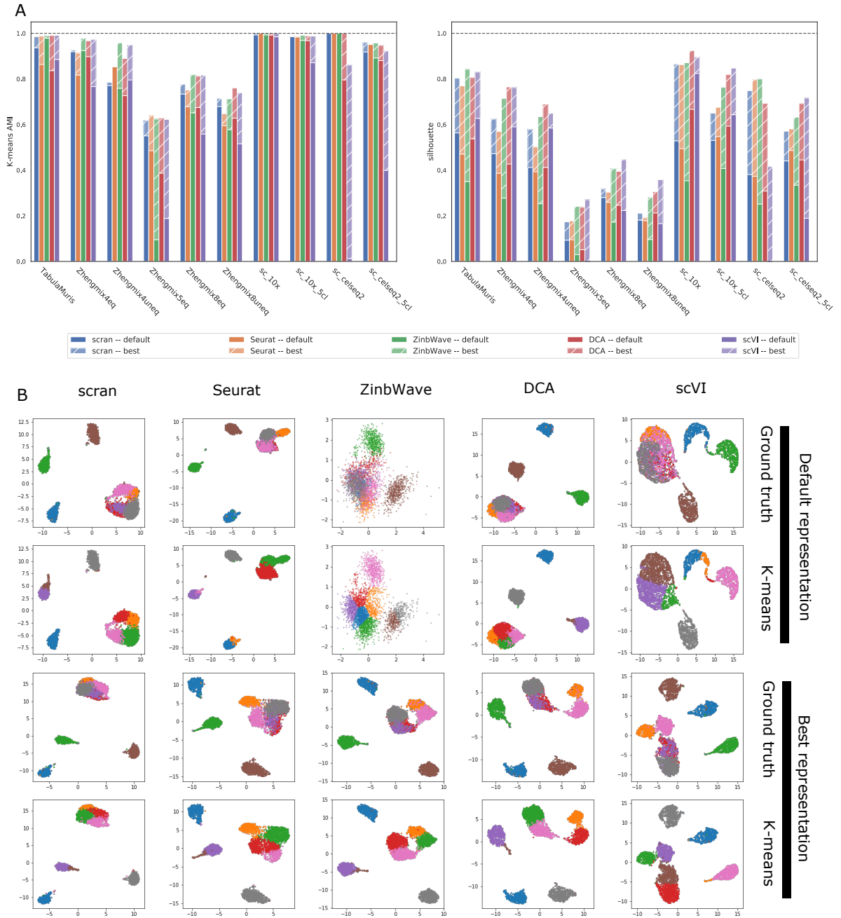
Figure 3.3: Performance of five DR pipelines (scrn, Seurat, ZinbWave, DCA and scVI) with default parameters and a dimension of 10 (legend "default") or after parameter optimization (legend "best") on our benchmark of ten datasets. A. AMI (left) and silhouette (right) reached by each method on each dataset. B. UMAP representation of Zhengmix8eq after DR by each method (in column) using default parameters (top two rows) of after parameter optimization (bottom two rows). In each row, cells are colored either based on their true cell type (rows 1 and 3) or based on a k -means clustering.
