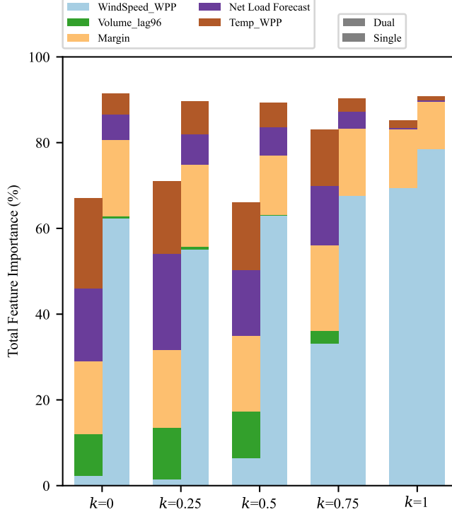
Figure 2.7: Normalized prescriptive feature importance for a subset of features.
