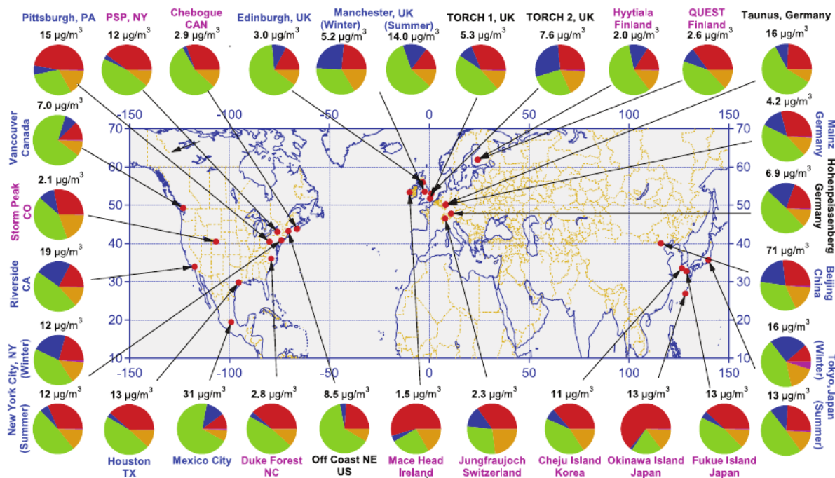
Figure 1.1: The chemical composition and concentrations of \text{PM}_{10} in the Northern Hemisphere. Source: [Zhang, 2007]
