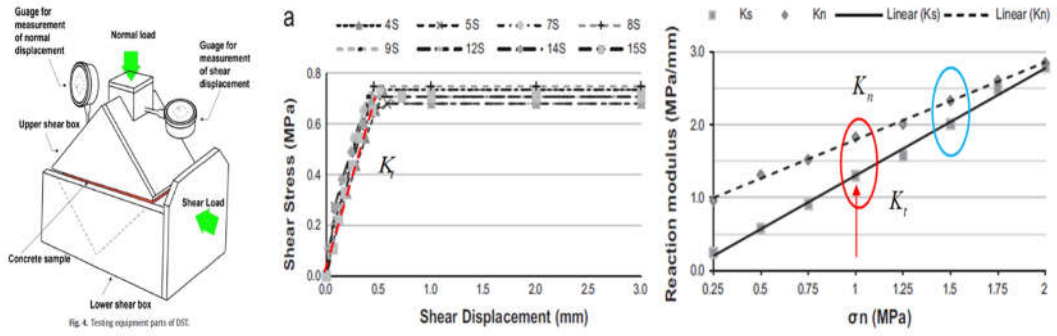
Figure 35. Experimental data on segment joint properties by SALEMI.A et al 2015 (Case -condition: the normal stress 1MPa without gasket)
