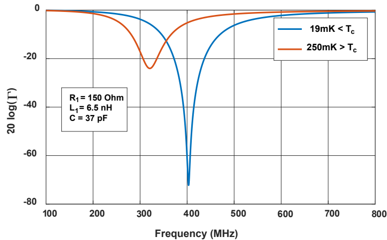
Figure 2.12: Magnitude of the reflection coefficient in dB of a LAO/STO(111) 2DEG, embedded in a RLC circuit which SMD R_1 and L_1 are specified in the figure. The red line correspond to the normal state signal where Z_{2DEG} = R_s and the blue one is the signal in the superconducting state where L_k is significant and shifts the resonance frequency \omega_0 = 1/\sqrt{(L_{tot}C_{STO})} .
