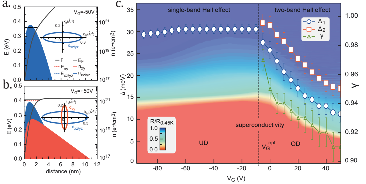
Figure 3.24: Superconducting phase diagram of the \text{LaAlO}_3/\text{SrTiO}_3(110) interface (sample A). a. and b. , Numerical simulations of the band structure in the (110)-oriented interface using self-consistent Poisson-Schrödinger equations for two doping regimes: V_G = -50 \text{ V} a. and V_G = +50 \text{ V} (b. same key as in a.) The confinement potential \phi in the energy scale as a function of the distance to the interface, the Fermi energy ( E_F ) and the energies of the different t_{2g} bands ( E_{xy} , E_{xz/yz} ) are shown on the left axis while the 3D carrier densities associated with each band ( n_{xy} , n_{xz/yz} ) are shown on the right axis. The 2D carrier density used in the simulation corresponds to the one reported on fig. 3.9, that is, n \approx 0.75 \times 10^{14} \text{ e} \cdot \text{cm}^{-2} at V_G = -50 \text{ V} and n \approx 1.1 \times 10^{14} \text{ e} \cdot \text{cm}^{-2} at V_G = +50 \text{ V} . The inset shows Fermi contours in the (k_z ([001]), k_M ([1-10])) plane for each gate voltage. c. , Gap energies \Delta_1(0) and \Delta_2(0) (left axis) and the individual stiffness weight \gamma (right axis) extracted from the fitting procedure, plotted as a function of V_G and superimposed on the sheet resistance colour map of fig. 3.7. Error bars correspond to the uncertainty in the fitting procedure.
