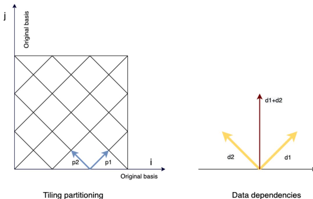
Figure 5.1: Tile partitioning
