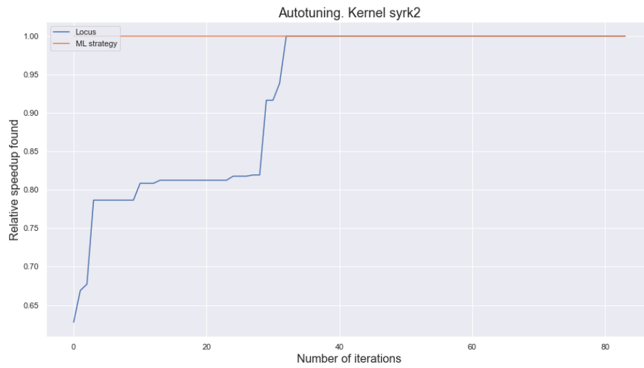
Figure 7.1: Syrk2 kernel
