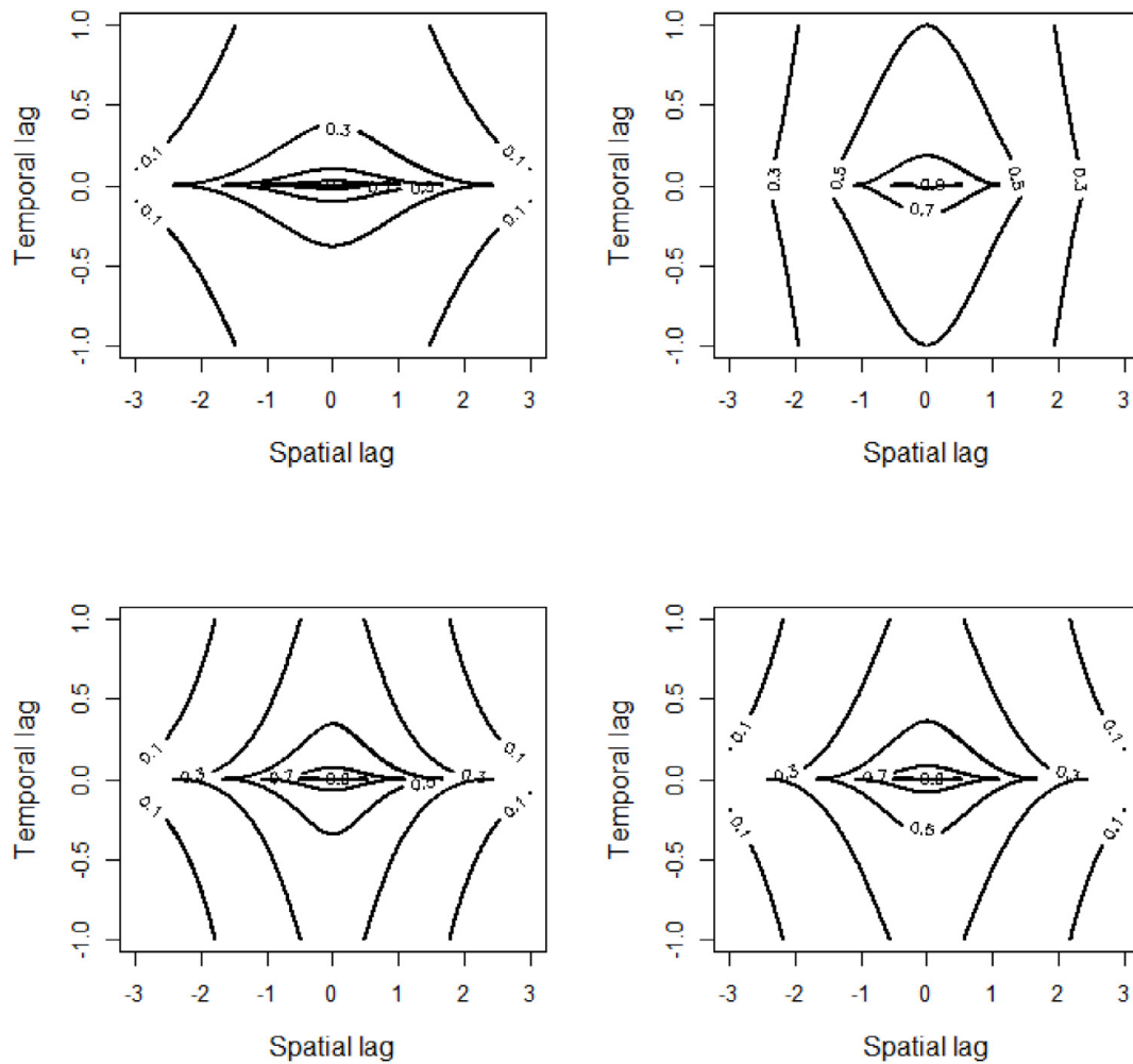
Fig. 1. Contour plots for the space-time covariance (15) with \eta(u) = \sqrt{|u|} , \nu = 1.5 , a^2 = b^2 = 1 : separability ((\alpha, \beta) = (1, 1)) , upper left), positive nonseparability ((\alpha, \beta) = (0, 1)) , upper right), negative nonseparability ((\alpha, \beta) = (1, 0)) , lower left) and general nonseparability ((\alpha, \beta) = (0.7, 0.3)) , lower right).
