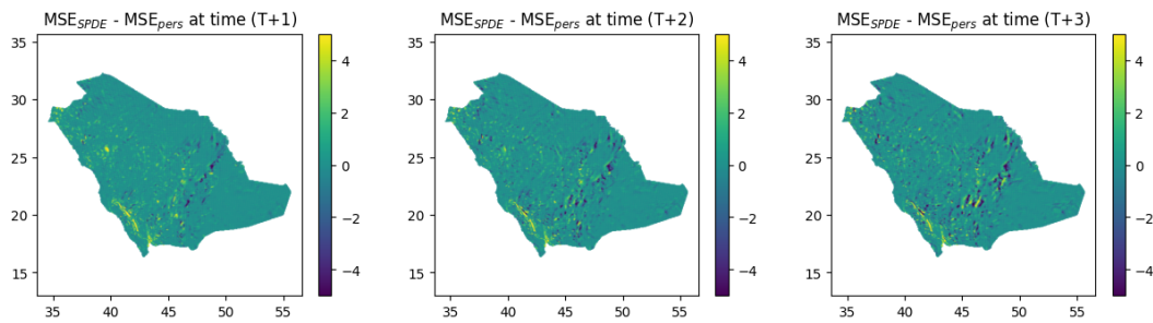
FIGURE 6.11: Difference between MSE of model (3) (regular mesh with N_S = 900 ) and MSE of persistence model at (T+1) , (T+2) and (T+3) .
