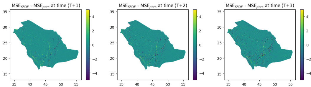
FIGURE 6.12: Difference between MSE of model (3) (handmade mesh with N_S = ) and MSE of persistence model at (T+1) , (T+2) and (T+3) .
