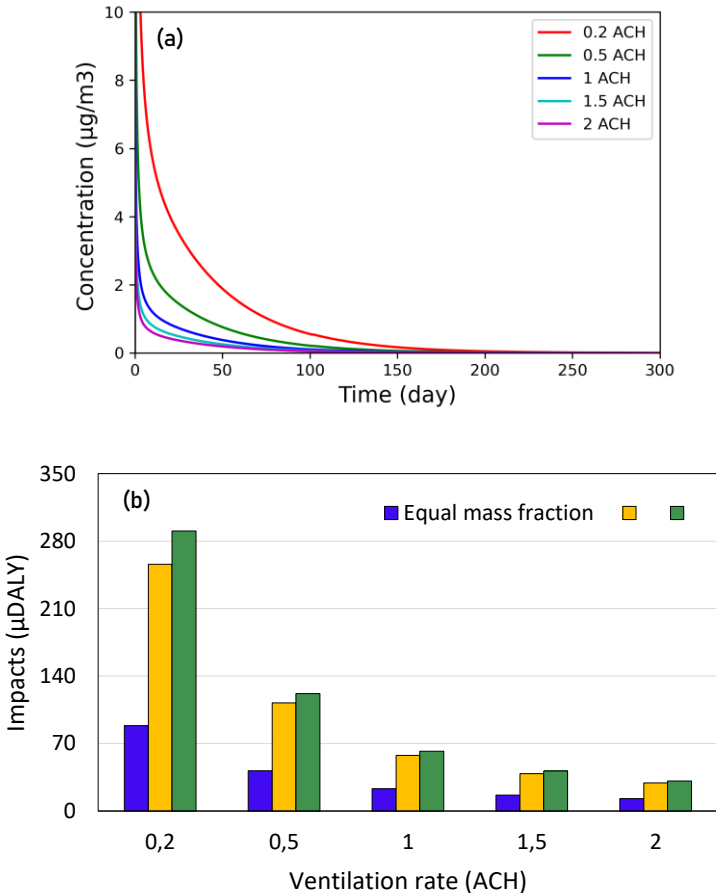
Figure 2-10: (a) Concentration curves for toluene emitted by gypsum board at different air changes per hour from 0.2 to 2 vol/h and (b) health damages related to the intake of VOCs emitted by gypsum board for different ventilation rates in the office
