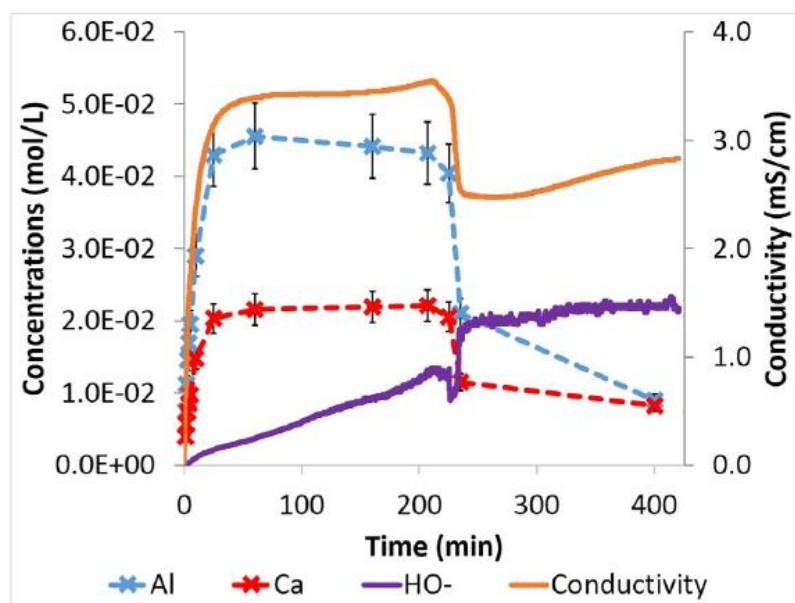
Figure 29 : Aqueous phase monitoring of the pure CA hydration at 10 \text{ g.L}^{-1} at 35 \text{ }^\circ\text{C} , reproduced from [151].
