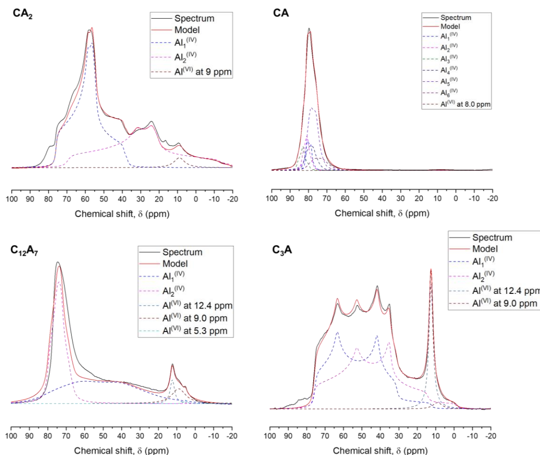
Figure 40 : ^{27}\text{Al} NMR spectra (black lines) and fit decomposition of the anhydrous phases with a second order quadrupolar lineshapes and of the octahedral Al sites of the hydrates with Lorentzian lineshapes [23].
