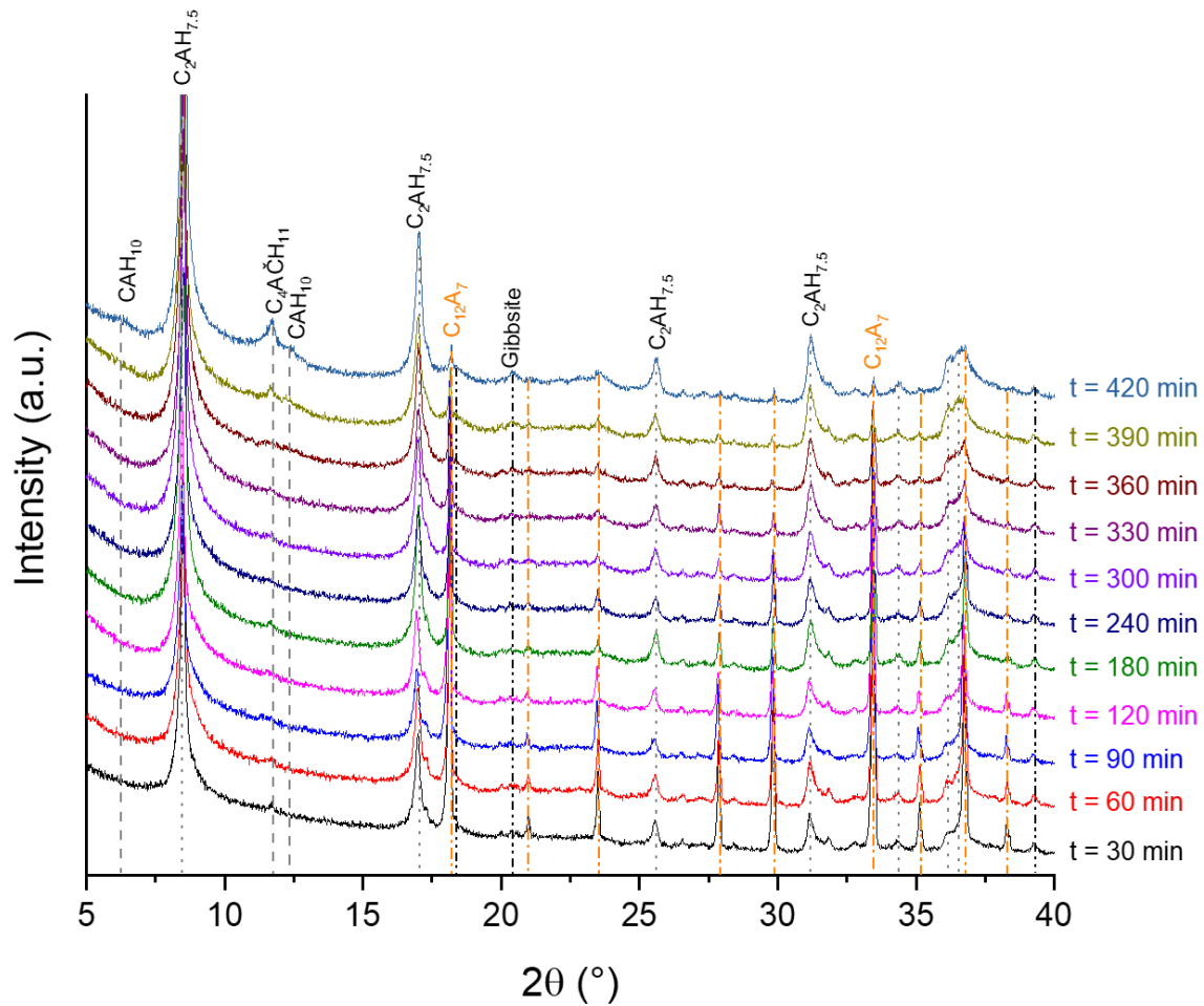
Figure 111 : XRD patterns of the solid fractions of C_{12}A_7 suspension with a w/c of 25 after increasing periods of hydration at 25 °C.
