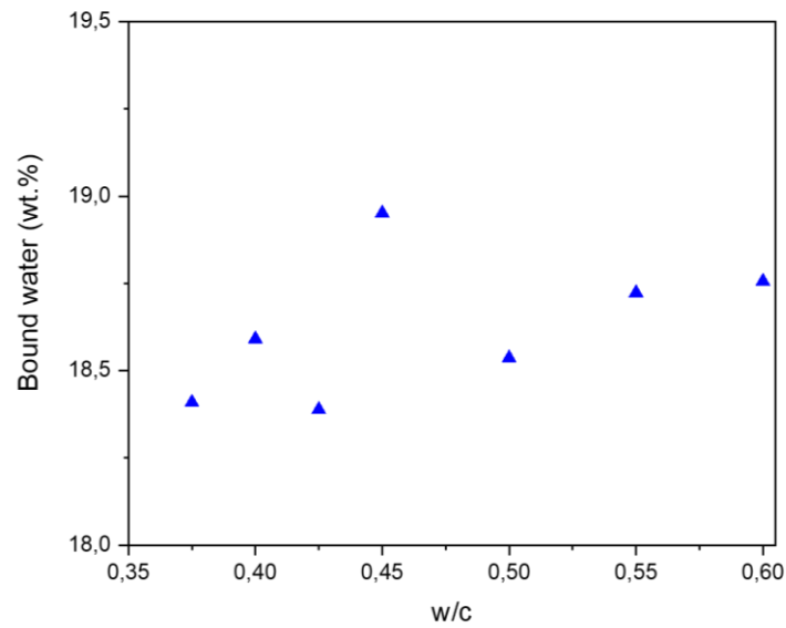
Figure 123 : Bound water amount of cubic- C_3A pastes with different w/c ratios hydrated at 25 °C for 7 days.
