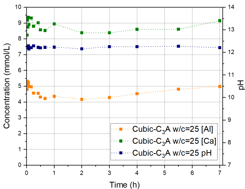
Figure 137 : Characterization of the liquid fractions of cubic- C_3A suspension (w/c ratio = 25, T = 25\text{ }^{\circ}C ) during the first seven hours of hydration: evolution of pH and chemical composition.
