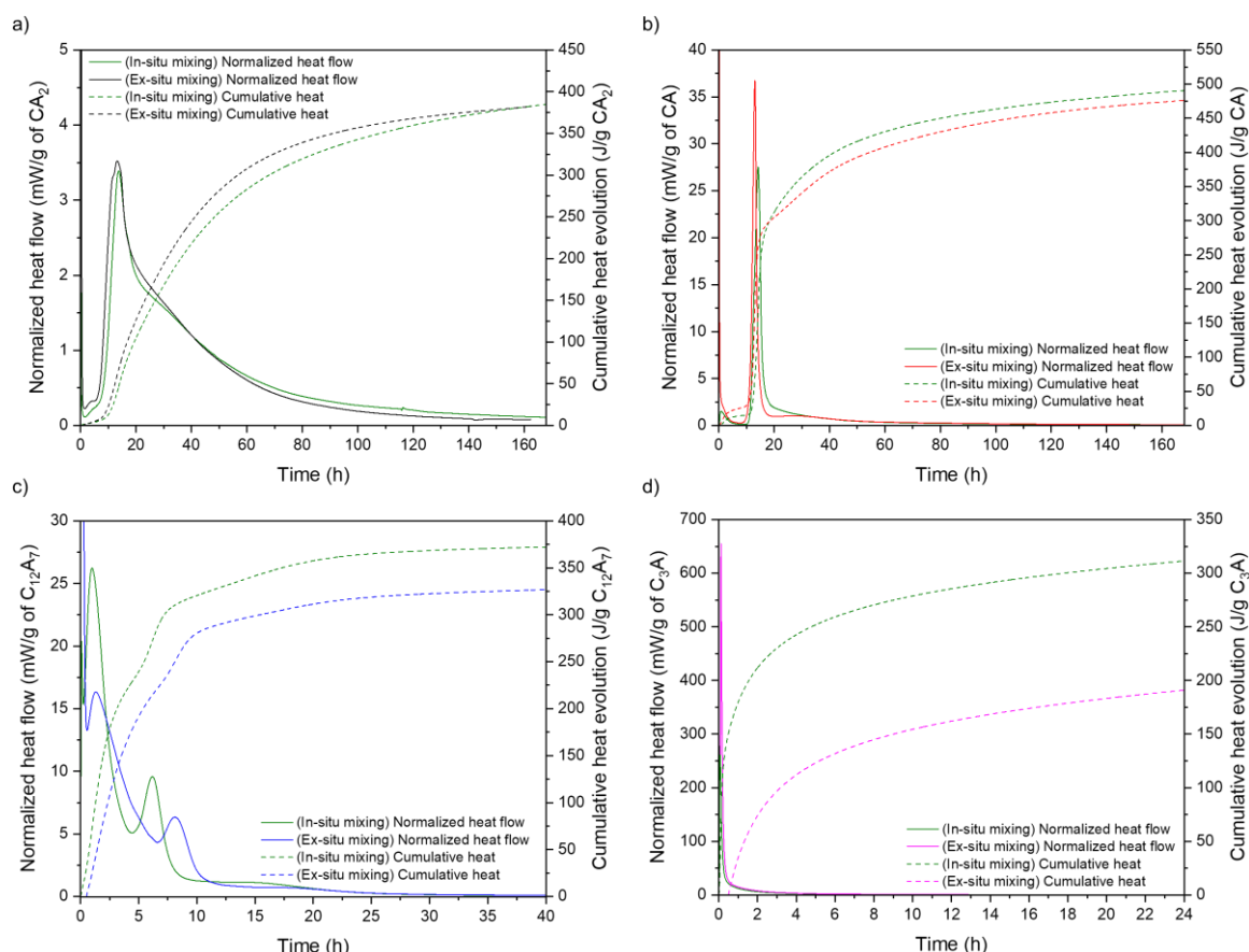
Figure 42 : Comparison of isothermal calorimetry measurements of the pastes ( w/c=0.5 ) prepared with the in-situ and ex-situ mixing methods at 25 °C for 7 days of hydration. a) CA_2 paste, b) CA paste, c) C_{12}A_7 paste and d) Cubic- C_3A paste (only results from the first 24 h of hydration monitoring).
