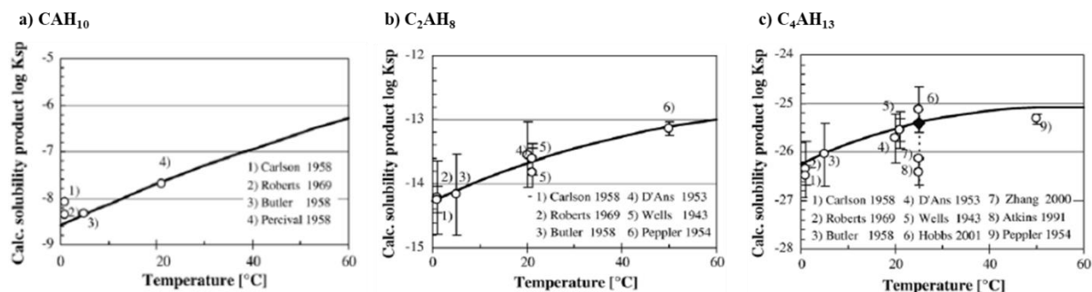
Figure 21 : Calculated temperature dependent solubility products of (a) \text{CAH}_{10} , (b) \text{C}_2\text{AH}_8 and (c) \text{C}_4\text{AH}_{13} , reproduced from [105].
