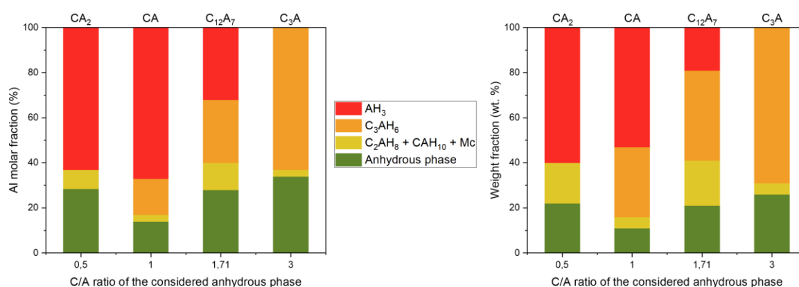
Figure 141 : Comparison between mineralogical assemblages achieved after seven days for each of the studied anhydrous phases – w/c = 0.5 – T = 25 °C. Estimation from ^{27}Al MAS NMR.
