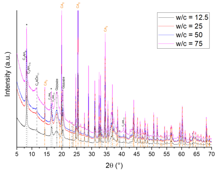
Figure 57 : XRD patterns representing mineralogical assemblages of CA 2 suspensions after 24 hours of hydration at 25 °C.
