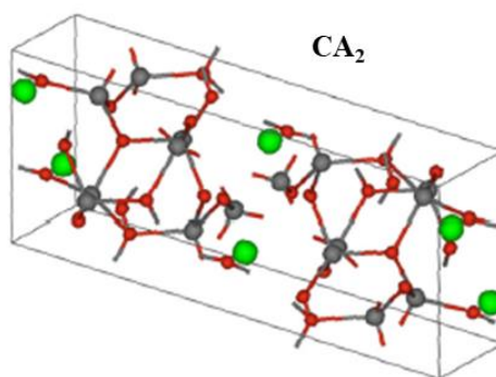
Figure 5 : Crystal structure of the CA_2 phase (Al, grey; Ca, green; O, red), reproduced from [20].
