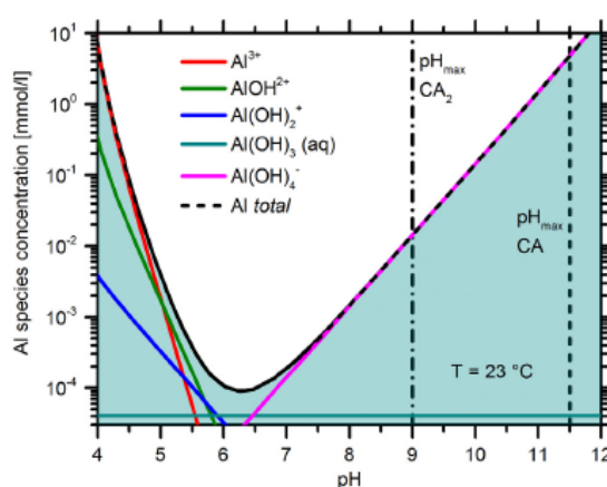
Figure 25 : Aluminium aqueous species distribution and equilibrium solubility curve of amorphous \text{Al}(\text{OH})_3 , reproduced from [111].
