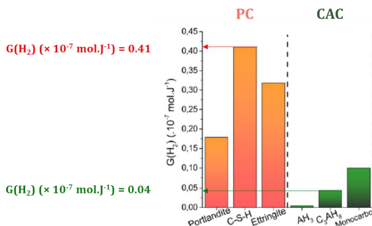
Figure 1 : G(H_2) values determined from Portland and Ciment Fondu® pastes and their hydrates, adapted from [9].
