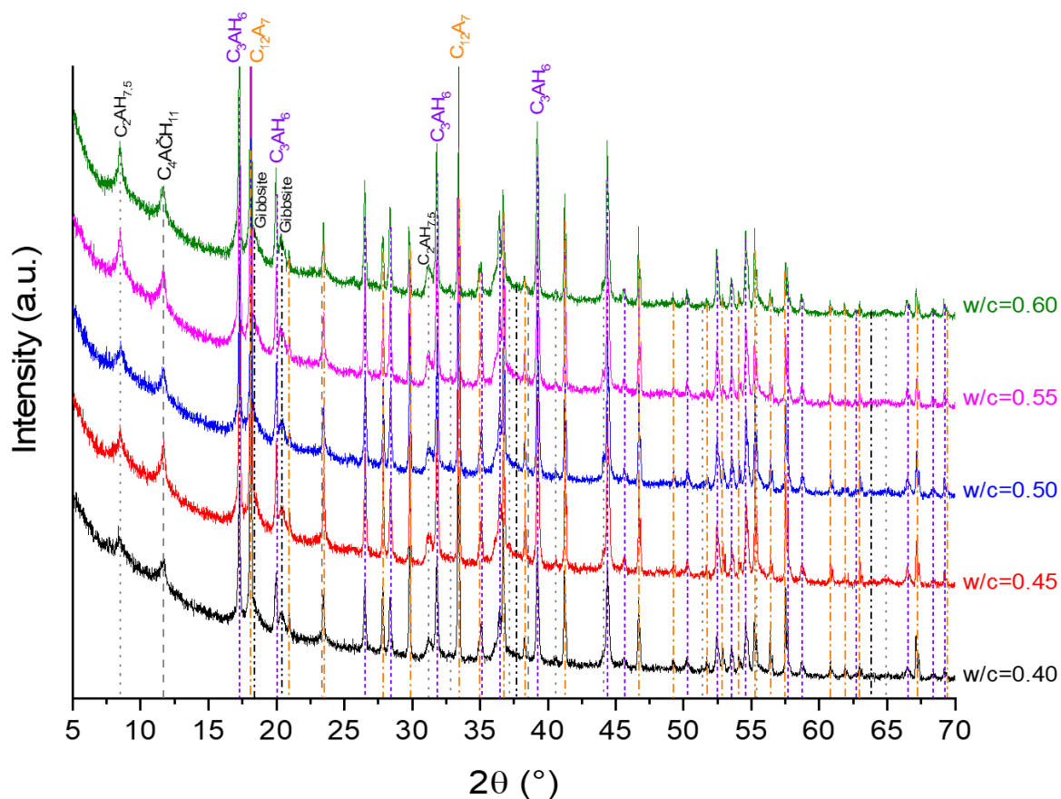
Figure 100 : XRD patterns representing hydration products after hydrating C 12 A 7 with w/c ratios ranging from 0.4 to 0.6 at 25 °C for 7 days.
