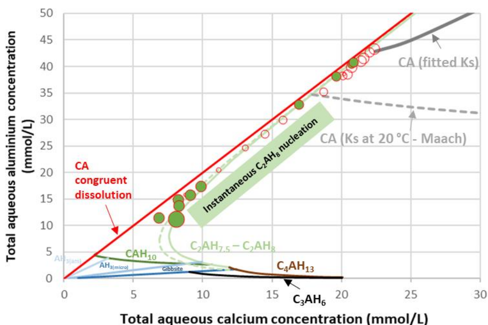
Figure 95 : Total calcium and aluminium concentrations measured in the liquid fraction during CA hydration ( w/c = 25 – T = 25\text{ °C} ) plotted in the \{CaO-Al_2O_3-H_2O\} phase diagram. Note that the red line is not a solubility curve. It simply shows the expected concentrations if the system is driven by congruent dissolution of CA.
