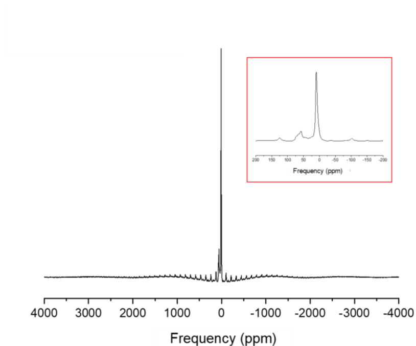
Figure 54 : ^{27}\text{Al} MAS NMR spectrum of the 7 d-old CA_2 paste ( w/c = 0.5 ).
