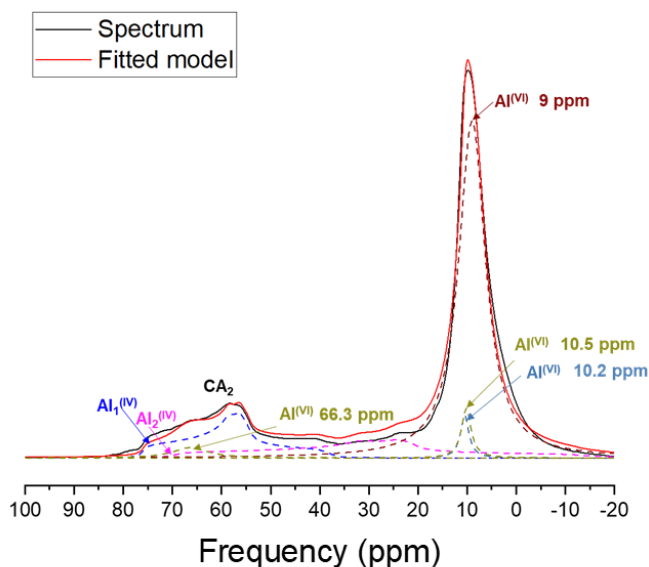
Figure 55 : Decomposition of the ^{27}\text{Al} MAS-NMR spectrum central bands of the 7 d-old CA_2 paste ( w/c = 0.5 ).
