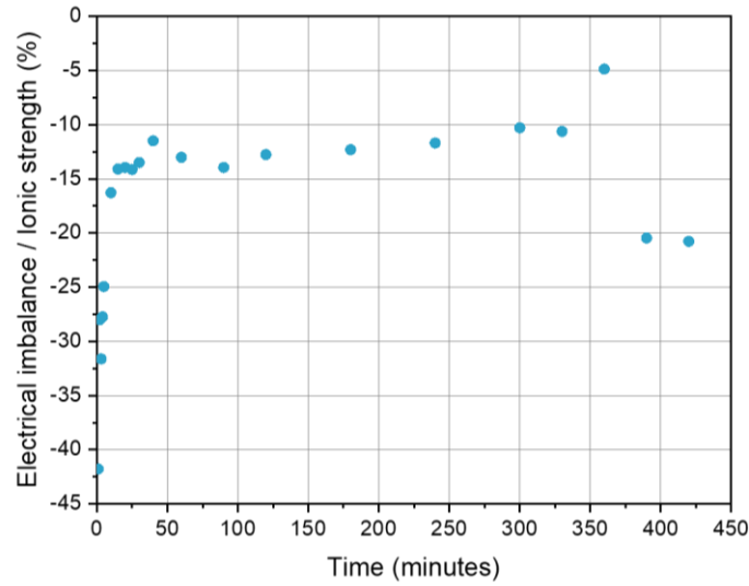
Figure 118 : Evolution of the electrical imbalance normalized by the ionic strength for the simulations carried out with CHESS and the CEMDATA2018 database as a function of the hydration time.
