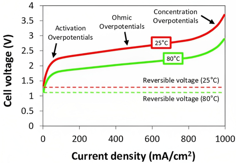
Figure 2.3: Schematic representation of a polarization curve of an alkaline electrolyzer at different temperatures, representing the voltage losses with current density, reprinted from [128].
