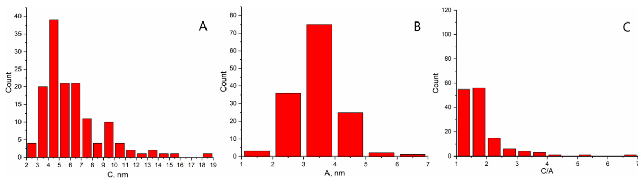
Figure 3.3. Left – distribution of particle long axes (C), middle – distribution of particle short axes (A), right – distribution of particle aspect ratios (C/A).
