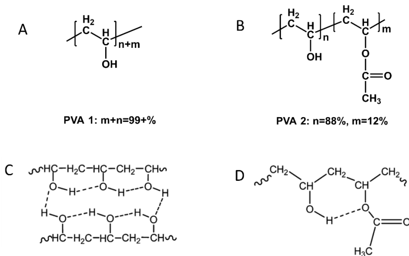
Figure 4.1. Chemical structure of PVA with different hydrolysis degrees. (A) PVA 1 is fully hydrolyzed with the DH ~ 99 % and (B) PVA 2 is less hydrolyzed with DH ~ 88 %. n is the number of repeated vinyl alcohol (VA-) groups and m is the number of vinyl acetate-(VAc-), in a PVA chain. (C) Hydrogen bonding associations for highly hydrolyzed PVA 3 . (D) Hydrogen bonding associations for partially hydrolyzed PVA 3 .
