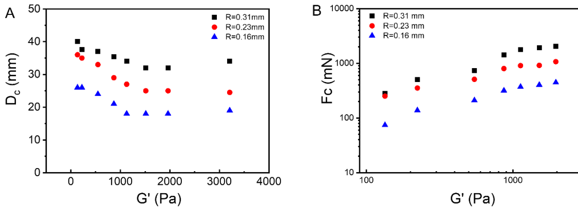
Figure 2.10. (A) Critical puncture displacement D_c and (B) critical puncture force F_c for PAAM hydrogel.
