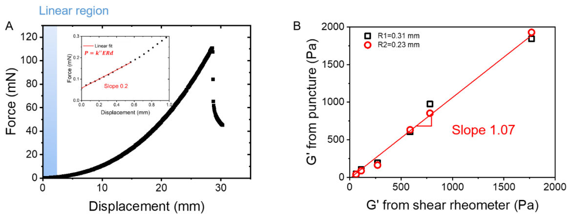
Figure 3.12. (A) Loading curve of PVA88 hydrogel from Path 1 ( G' = 250 Pa and R = 0.23 mm) with an indicated linear region in blue shadow (the inset shows the linear fitting of the Neo-Hookean model). (B) Comparing elastic modulus from puncture experiment (with indenter R = 0.31 mm and R = 0.23 mm for examples) and rheology.
